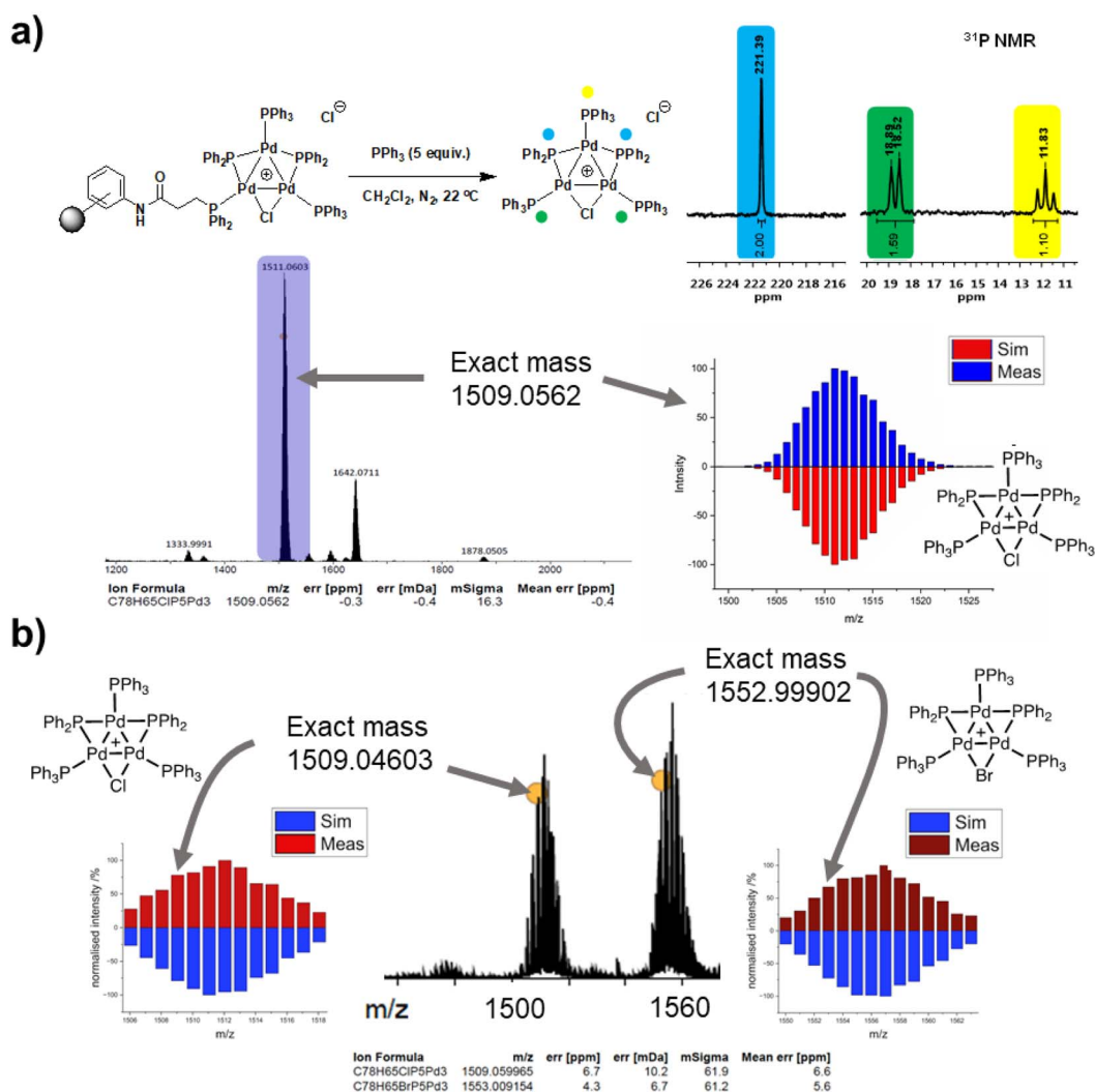
Fig. 6 (a) Reaction of immob-Pd 3 Cl 2 3 with 5 equiv. PPh 3 in CH 2 Cl 2 at 22 °C; 31 P NMR spectrum was recorded upon dissolution (within 10 min). ESI-MS (+ve mode) confirms pseudo-molecular ion at m/z 1509, with the correct isotopic distribution pattern centered at m/z 1511 (bottom right); (b) ESI-MS (+ve mode) analysis of the solution after reaction of excess PPh 3 with post-reaction immob-Pd 3 Cl 2 3 cluster which was filtered off 10 minutes into Suzuki–Miyaura catalytic turnover and thoroughly washed, showing both [Pd 3 Cl] + and [Pd 3 Br] + ions shown, with their correct isotopic distribution patterns.
