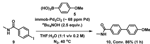
Scheme 2 Control SMCC of 4-iodo- N -methylbenzamide 9 with 4-methoxyphenyl boronic acid 5 , catalyzed by immob-Pd 3 Cl 2 3 .
