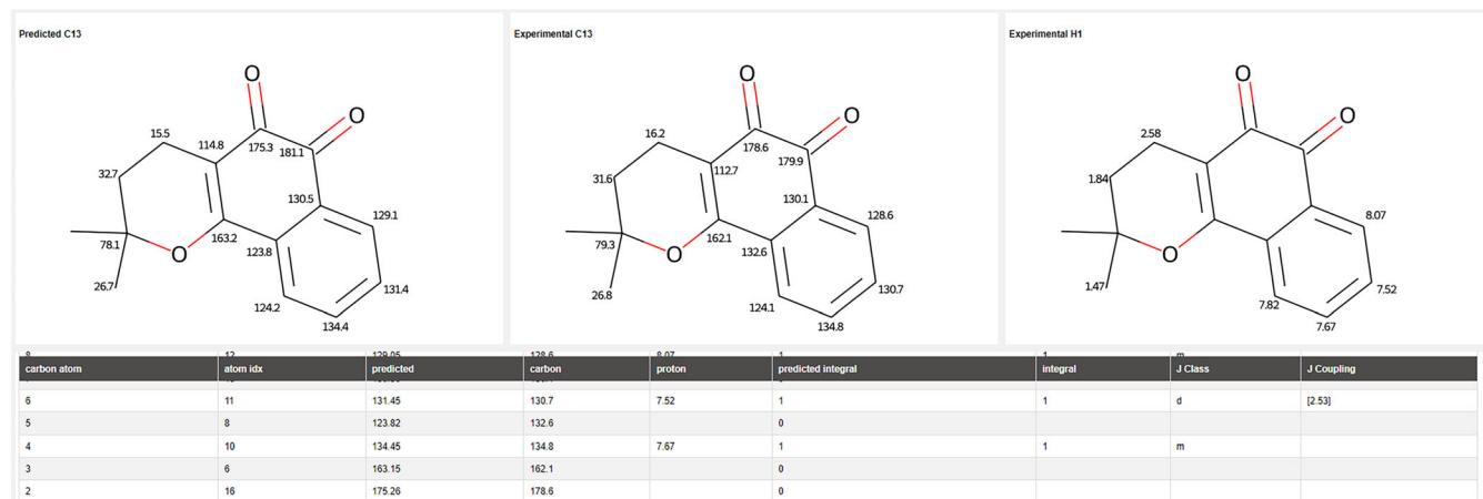
FIGURE 6 Report for the (corrected) assignment of beta-Lapachone, showing the significant discrepancy between the predicted and observed ^{13}\text{C} chemical shift for carbon atom 5, one of the quaternary aromatic carbons
