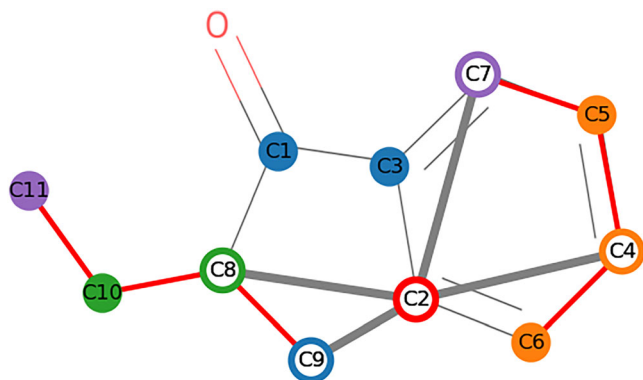
FIGURE 4 Positioning of CH x fragments completed, with the mouse pointer hovering over one of the quaternary aromatic carbons (C2) showing the characteristic three-bond HMBC correlations in the aromatic ring
