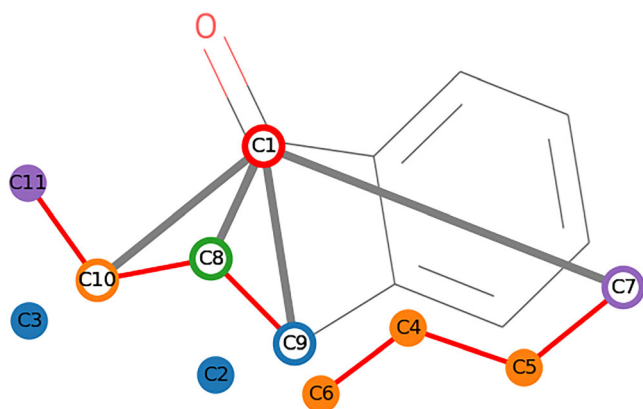
FIGURE 3 HMBC correlations to the carbonyl carbon
