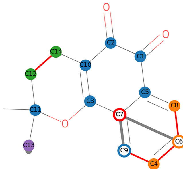
FIGURE 5 Assignments for beta-Lapachone based on 13 C chemical shift predictions using the NMRShiftDB2 software. The mouse cursor is hovering over the quaternary aromatic carbon, C7, and showing (probably erroneous) two- and four-bond HMBC correlations. This can be readily rectified by interchanging C7 with the adjacent C5. A movie of this process is provided in Movie S2.
