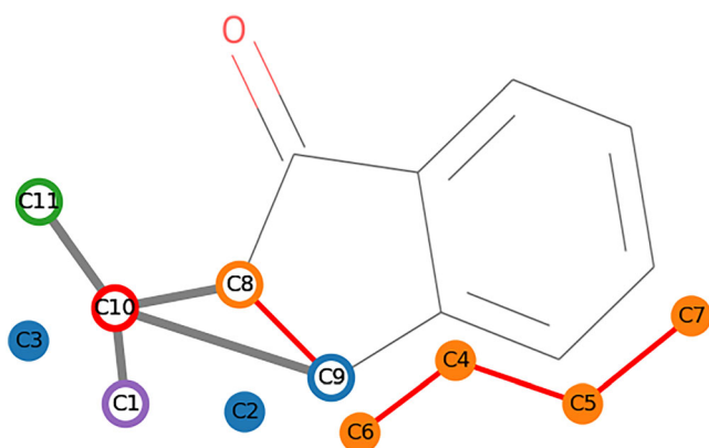
FIGURE 2 Situation after initial placement of COSY linked fragment of 2-ethyl-1-indanone with the mouse pointer hovering over the methylene group adjacent to the methyl group
