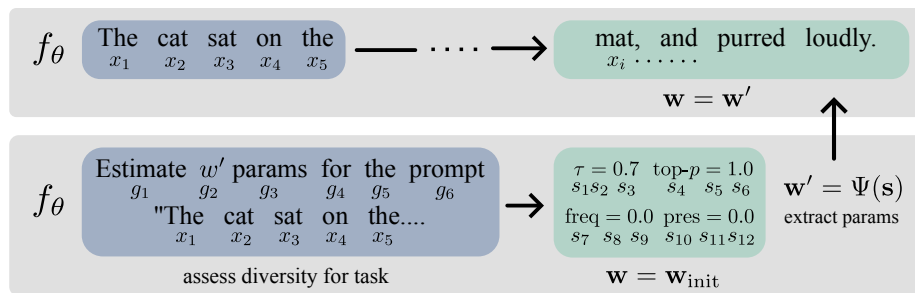
Figure 1: For a given task x = \text{"The cat sat on the"} , we guide the LLM f_\theta to generate a string of diversity parameters s = \text{"}\tau = 0.7, \dots \text{"} , which are then injected back into the subsequent sampling of f_\theta before completing the task x .
