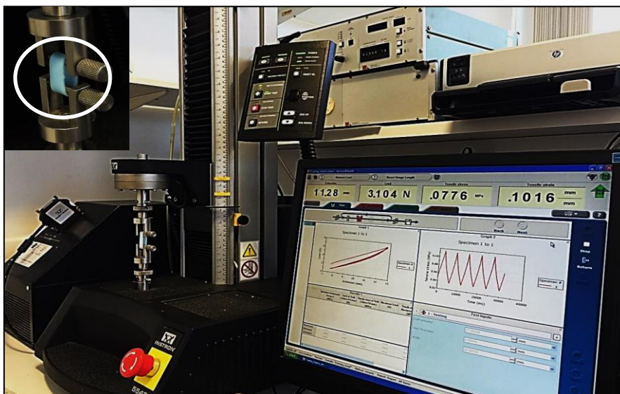
Fig. 4. Setup of Instron machine that used to perform the tensile tests for the manufactured silicone parts.
