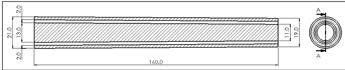
Fig. 2. Technical drawing for the assembled 3D printed mold of the abdominal aorta. All dimensions shown are in (mm) as shown in Table 1.
