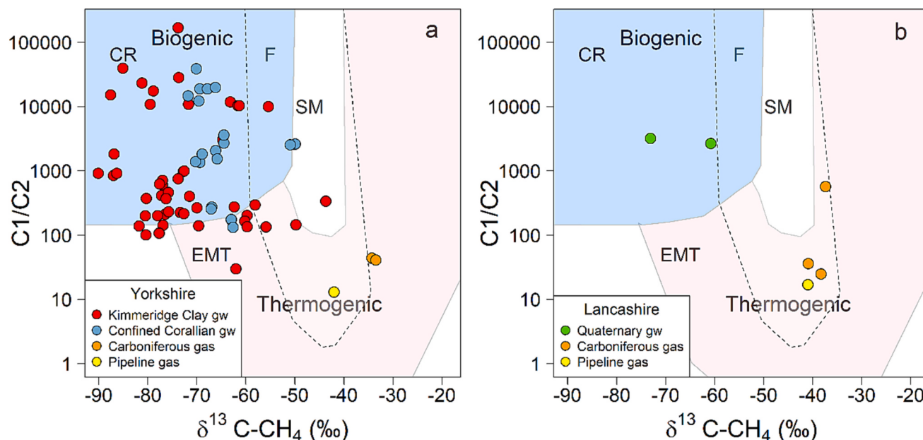
Fig. 5. Molar ratios of methane/ethane ( C_1/C_2 ) against \delta^{13}C-CH_4 in groundwater (gw) as well as free gas from Carboniferous hydrocarbon boreholes and atmospheric emissions from gas pipeline leaks in (a) the Vale of Pickering, Yorkshire and (b) Fylde, Lancashire. Carboniferous gas data for the Vale of Pickering are from conventional gas boreholes, those for Fylde are from Preese Hall shale-gas exploration borehole. Data for pipeline gas for each area are from Lowry et al. (2020). Discriminant fields for biogenic and thermogenic methane are also shown, along with fields for CR: CO_2 reduction, F: fermentation, SM: secondary microbial (petroleum biodegradation), EMT: early mature thermogenic (fields from Milkov and Etiope, 2018).
