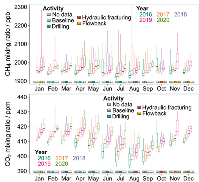
Fig. 4. Boxplots for monthly CH 4 (ppb) and CO 2 (ppm) mixing ratios measured under westerly winds ( 270^\circ \pm 45^\circ ) at PNR. Boxplots in different colours represent the different years of data between February 2016 and September 2020. For each boxplot, the thick line represents the monthly median mixing ratio, the outer edges of the box represent the interquartile range, and the upper and lower whiskers extend to the 10th and 90th percentile values respectively. The coloured rectangles below the boxplots provide an indication of the reported activities taking place at PNR during each month. A blank rectangle indicates that there were no reported activities; © 2024 University of Manchester.
