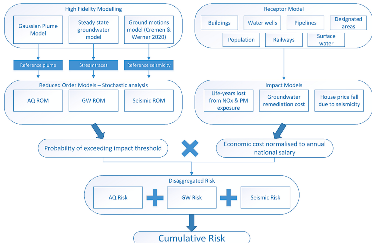
Fig. 3. Flowchart of the risk-assessment methodology; AQ: Air Quality, GW: Groundwater, ROM: Reduced-Order Model; © 2024 University of Edinburgh.
