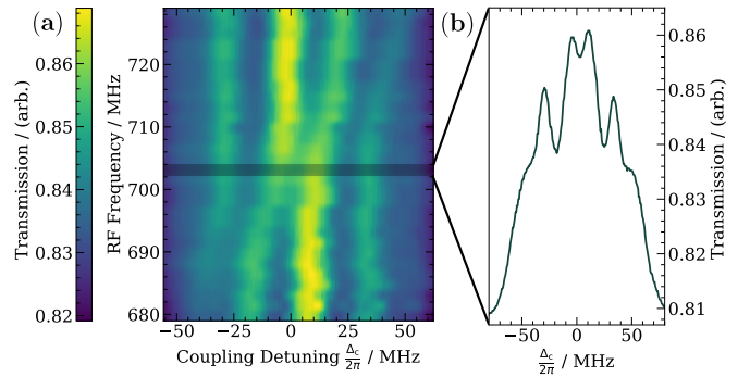
FIG. 3. Spectral map of the I \rightarrow K transition as the RF field is swept and coupling laser is detuned across resonance. (a) A color map made up of the resultant probe transmission traces in response to scanning the RF field over resonance for the 17I \rightarrow 17K transition at \sim 700 MHz. (b) A plot of the probe transmission against the coupling detuning for an RF field of 0.703 GHz - a grey bar shows the EIT trace which makes up that respective part of the color map.
