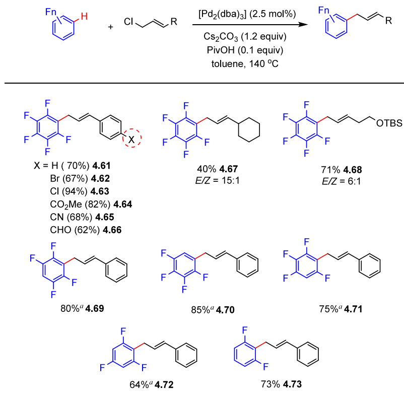
Scheme 22. Palladium-Catalyzed Allylation of Fluoroarenes with Allylic Chlorides 147
