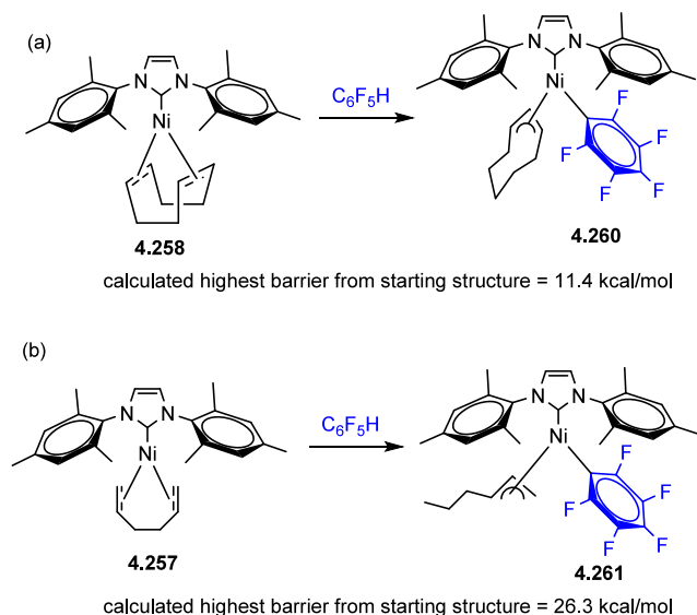
Scheme 53. Formation of \pi -Allyl Nickel Complexes As Off-Cycle Intermediates via Hydride Migration from Fluoroarenes 208
