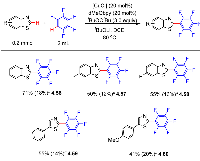
Scheme 20. Copper-Catalyzed Dehydrogenative Cross-Coupling of Benzothiazoles with Pentafluorobenzenes 140
