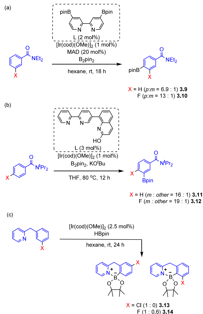
Scheme 7. Selected Examples of C–H Borylation Regioselectivity Enhanced by an ortho Fluorine Substituent a121–123
