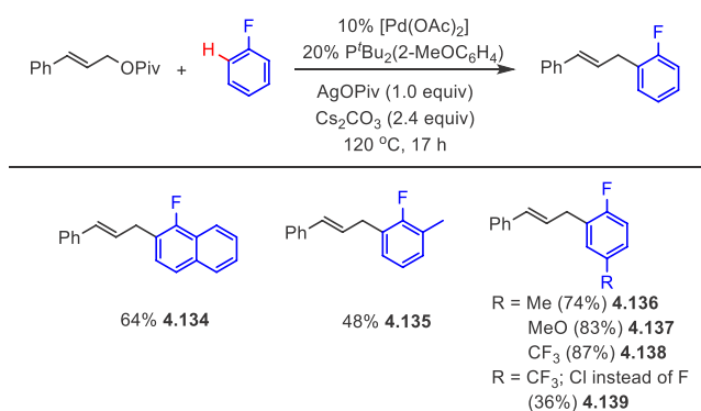
Scheme 33. Scope of the Palladium-Catalyzed C–H Allylation of Monofluoroarenes with Cinnamyl Pivalate 90
