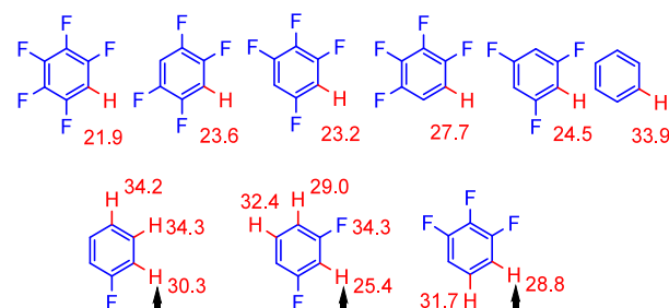
Figure 3. Gibbs free energies of activation ( \Delta G^\ddagger(298\text{ K}) in kcal/mol) of C–H bonds in different fluorinated arenes by [\text{Pd}(\text{C}_6\text{H}_5)(\text{PMe}_3)(\text{OAc})] via the CMD/AMLA process. For the three fluorobenzenes below, the arrow shows the position with the lowest barrier. 63
