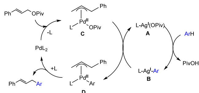
Scheme 35. (a) Palladium-Catalyzed Carbonylative Cross-Coupling of 4-Bromoanisole with Various (Poly)fluoroarenes and (b) Synthesis of a 13 C-Labelled NOS Inhibitor 162
