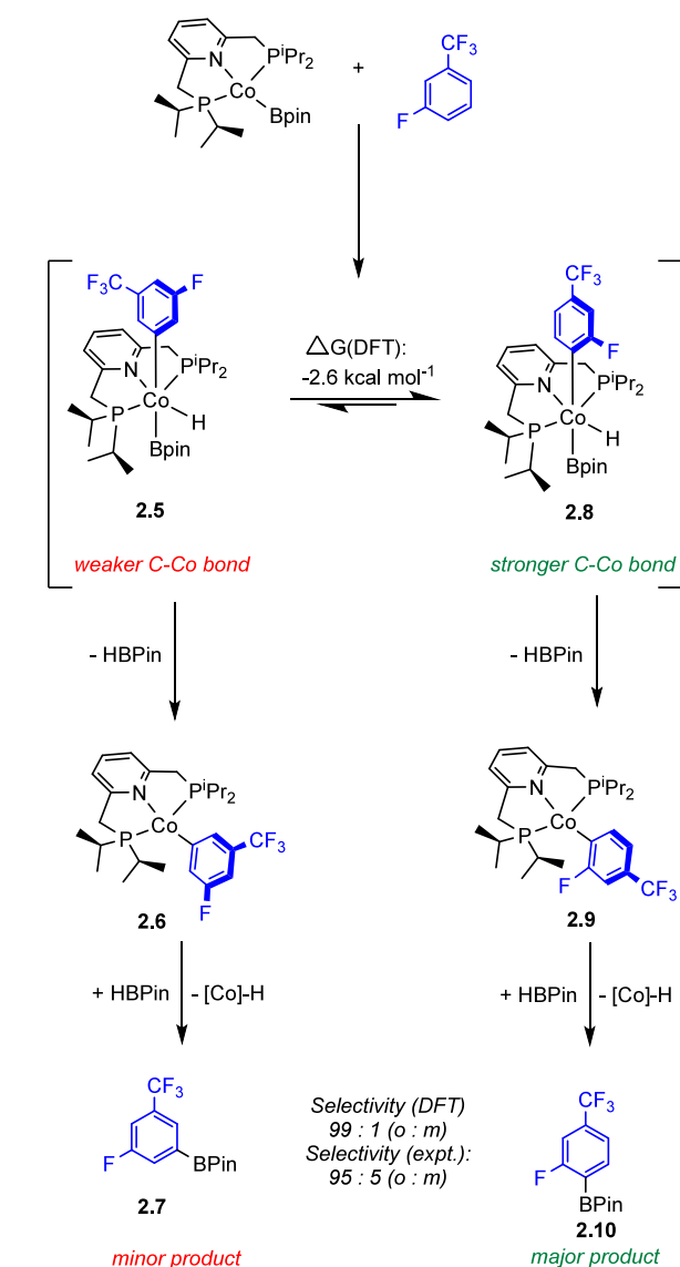
Scheme 2. Thermodynamic Control of C–H Oxidative Addition in Cobalt-Catalyzed ortho to Fluorine C–H Borylation 72
