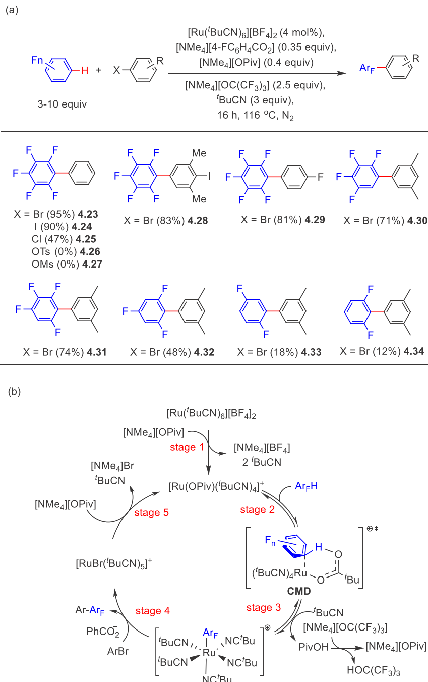
Scheme 14. (a) Ruthenium-Catalyzed Arylation of (Poly)fluoroarenes with Aryl Halides and (b) Proposed Catalytic Cycle 131
