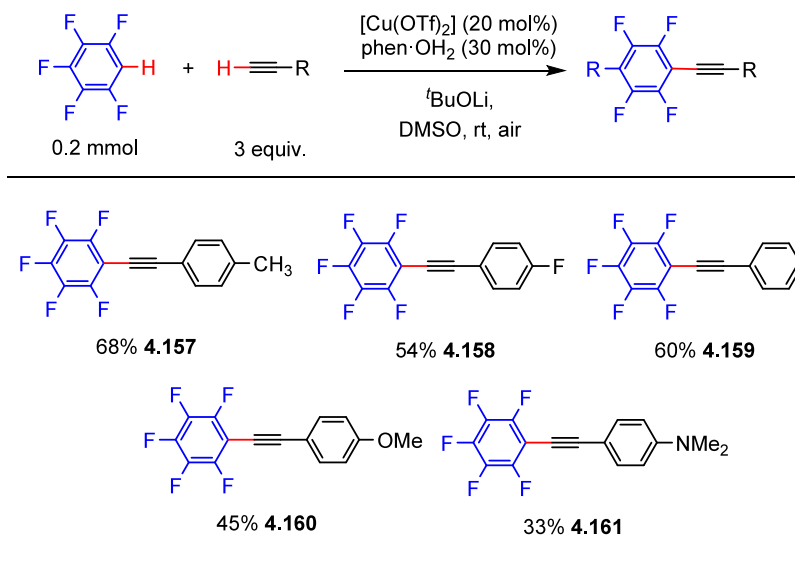
Scheme 39. Palladium-Catalyzed Benzylization of (Poly)fluoroarenes 169
