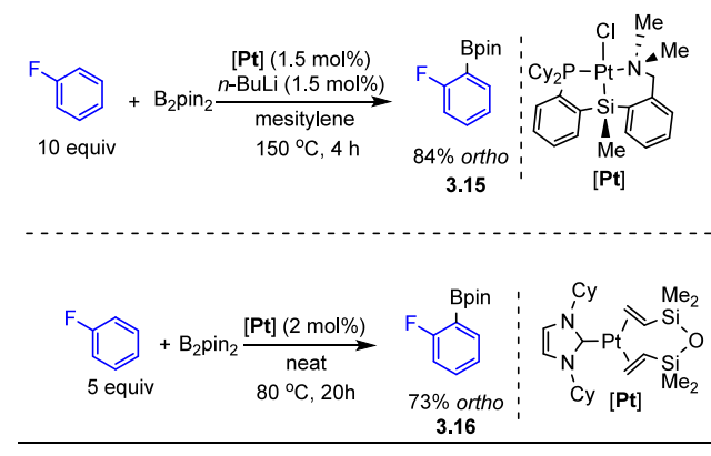
Scheme 8. Platinum-Catalyzed C–H Borylation of Fluoroarenes 54,55,119
