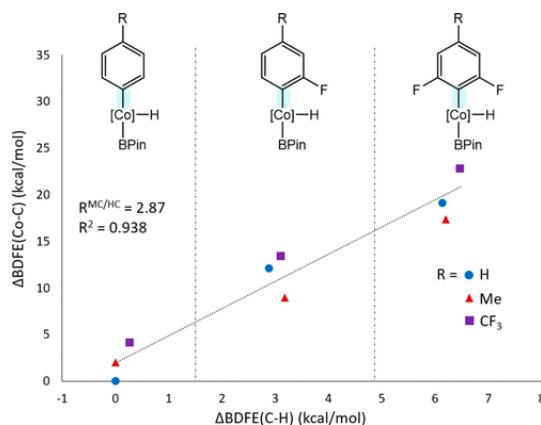
Figure 2. (a) Calculated contributions to Rh–C bond dissociation energy in kJ/mol from ortho and meta/para fluorine substitution for [CpRh(PH 3 )(H)(Ar F )]. Each point represents a different fluorinated benzene. The straight line represents the function in eq 1. Reproduced with permission from ref 71. Copyright 2009 American Chemical Society. (b) Correlation between the Co–C bond dissociation free energies (BDFEs) of the type represented by 2.5 and 2.8 and the C–H BDFEs in kcal/mol of the corresponding arenes. The zero points for the x - and y -axes correspond to the values for the C–H BDFE in benzene and the Co–C BDFE in the phenyl analogue of 2.5, respectively. Reproduced with permission from ref 72. Copyright 2019 American Chemical Society. Note the way that the points fall into groups for 0, 1, or 2 ortho fluorines in both graphs.
