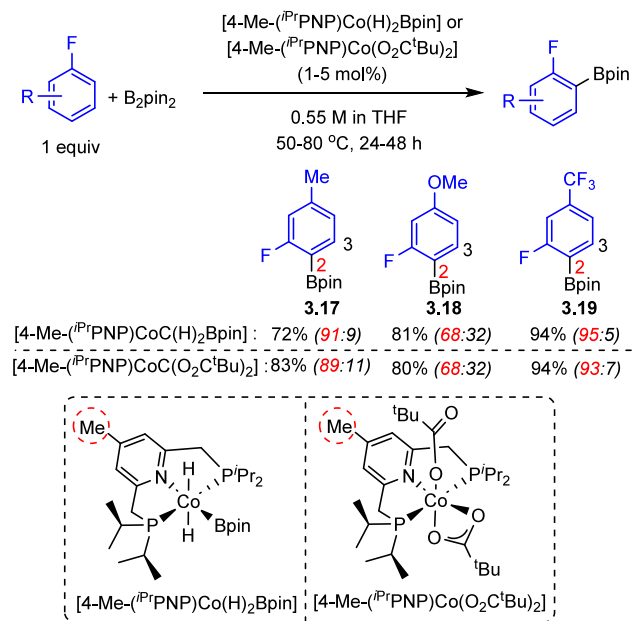
Scheme 9. Cobalt-Catalyzed ortho -to-Fluorine C–H Borylation 118
