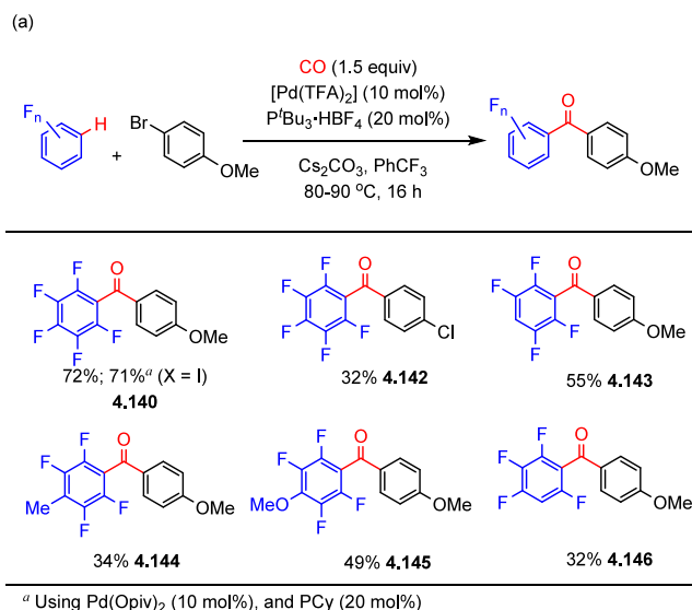
Scheme 35. (a) Palladium-Catalyzed Carbonylative Cross-Coupling of 4-Bromoanisole with Various (Poly)fluoroarenes and (b) Synthesis of a 13 C-Labelled NOS Inhibitor 162
