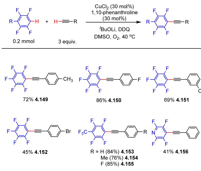
Scheme 37. Copper-Catalyzed Direct Alkynylation of (Poly)fluoroarenes with Terminal Alkynes 167
