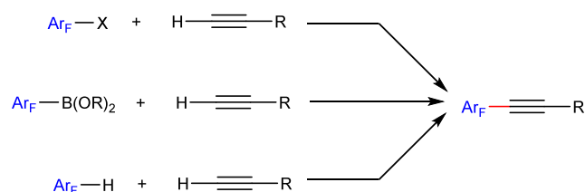
Scheme 36. Three Different Routes to Synthesize Aryl Alkynes
