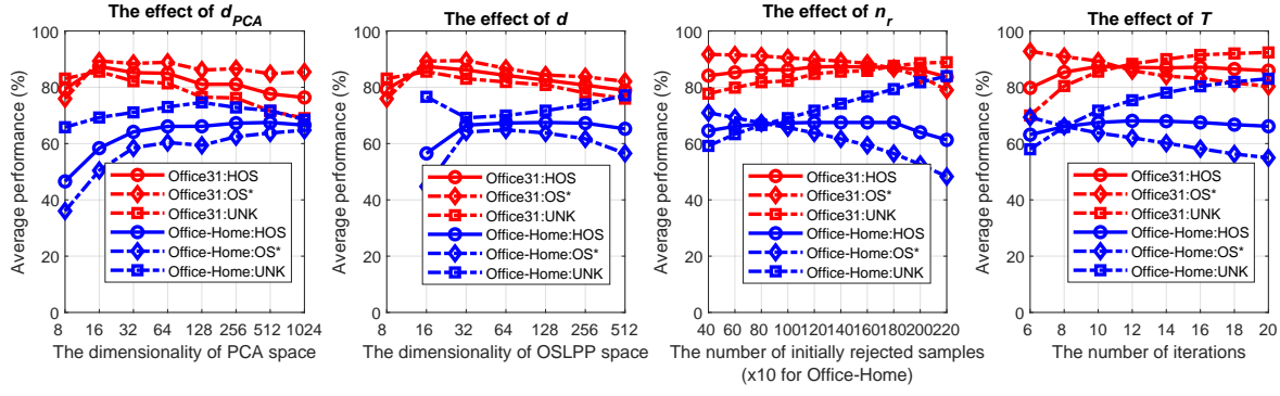
Fig. 3. The effect of hyper-parameters on the Office31 and Office-Home datasets.
