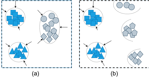
Fig. 1. An illustration of the motivations of our proposed approach (marker shapes represent different classes; known classes and unknown classes are represented by the blue and grey colours respectively; the arrows represent the explicitly optimized objectives during subspace learning). (a) Existing approaches tend to push all the unknown classes together when learning the (C+1) -class classifier; (b) we relax the constraint by only pushing the known classes together and the remaining unknown classes will be relatively far away from these known class clusters.
