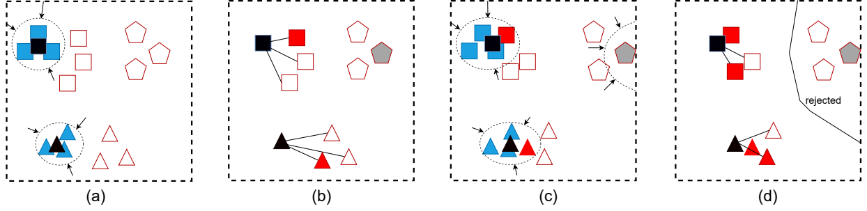
Fig. 2. An illustration of our proposed approach to OSDA. The blue and red colours are used to represent the source and target domains, respectively; different shaped markers represent different classes; the black markers are the class means; the hollow red markers are unlabelled target samples which are filled in with the red colour if selected as known classes and filled in with the grey colour if rejected as unknown classes. (a) A supervised LPP is applied to the labelled source data to pull the source samples from the same class closer to each other. (b) In the subspace learned by (a), class means are computed and used to selectively assign pseudo-labels to the target samples; on the other hand, target samples far away from all class means are rejected as unknown classes. (c) Our proposed OSLPP is applied to the labelled source samples, selected pseudo-labelled target samples and rejected target samples so that the samples from the same class regardless of their domains are pulled close to each other whilst those rejected as unknown classes are pushed away from the known classes. (d) In the subspace learned by (c), class means are computed and used to selectively assign pseudo-labels to the known classes; the target samples are rejected if their nearest neighbour is already rejected. Steps (c) and (d) are repeated for T times.
