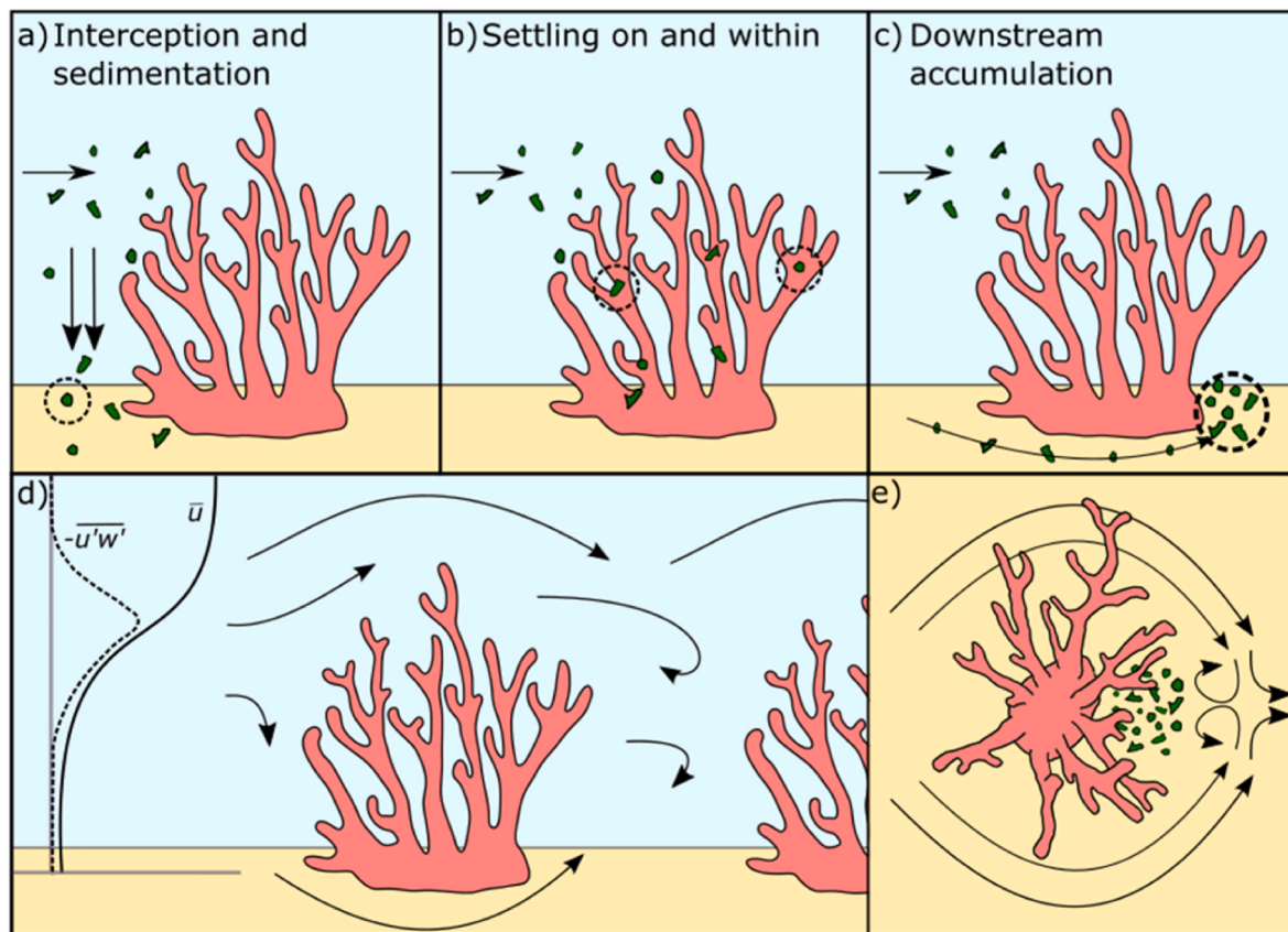
Fig. 6. (a–c) coral microplastic trapping mechanisms, and (d–e) the associated fundamental hydraulic profiles and flow contours (arrows) as supported by supplementary video 1.
