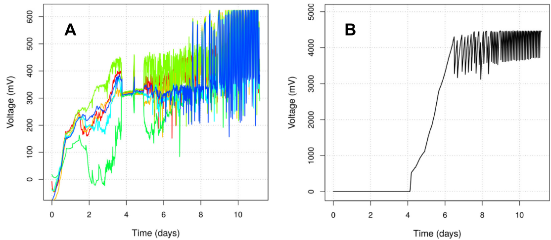
Figure 9. Results of the experiments testing the voltage produced by the microbial fuel cells. (A): Voltage produced by each of the six microbial fuel cells (various colours) and (B): Voltage gathered by the super-capacitor charged by microbial fuel cells (black). Figure Reproduced from [14]. CC BY 4.0.
