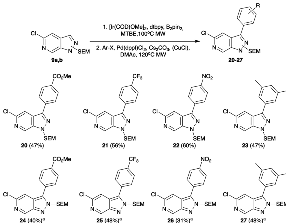
Scheme 3 Tandem C-H borylation and Suzuki-Miyaura cross-coupling of 9 . Conditions: (1) [\text{Ir}(\text{COD})\text{OMe}]_2 , dtbpy, \text{B}_2\text{pin}_2 , MTBE, 100^\circ\text{C} , MW, (2). Ar-X, \text{Pd}(\text{dppf})\text{Cl}_2 , \text{Cs}_2\text{CO}_3 , DMAc, 120^\circ\text{C} , MW. a Additional CuCl.
