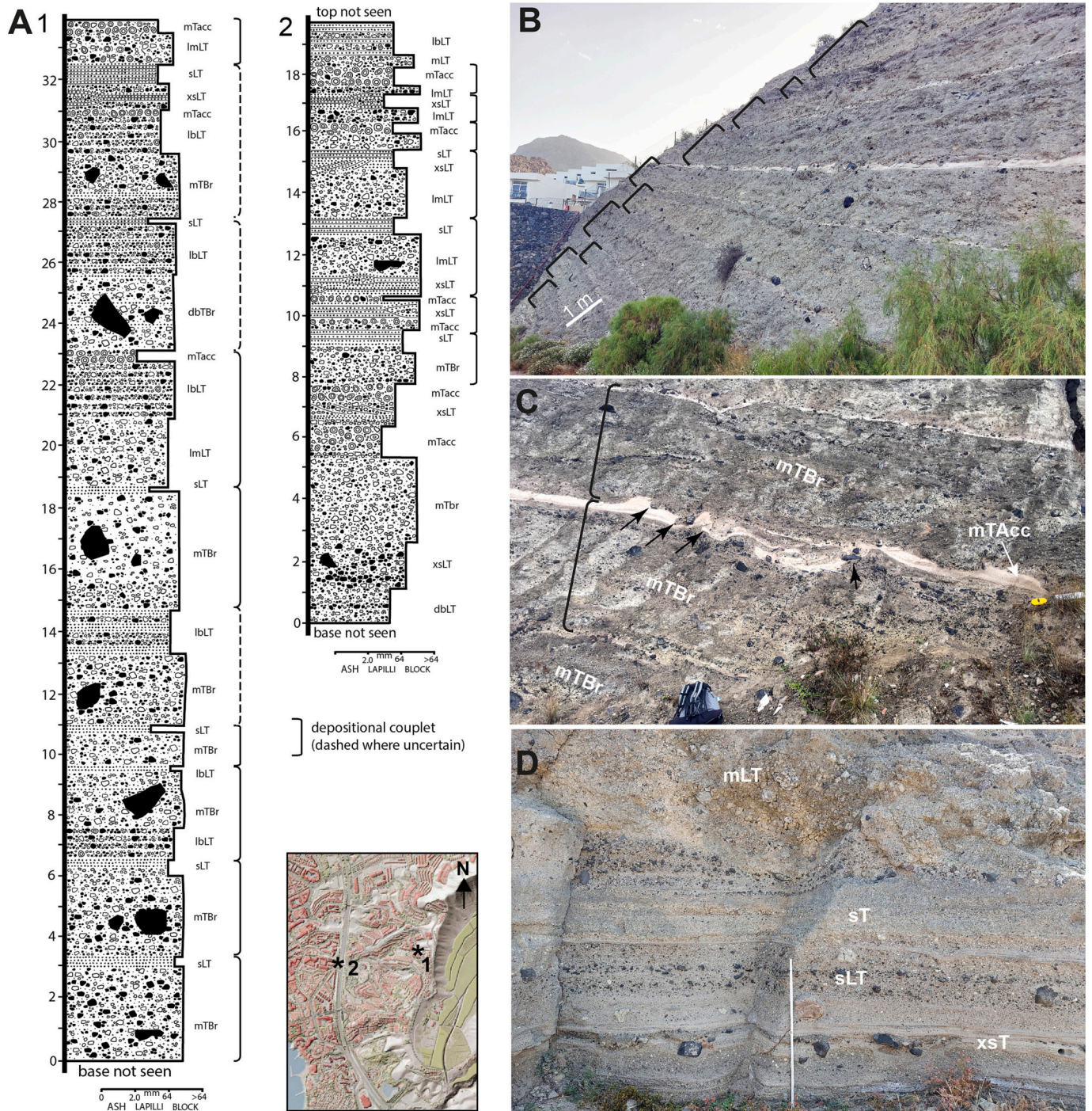
Fig. 8. Member E. A) Measured sections through Member E. Inset map shows location of logs. B) Depositional couplets consisting of thick beds of massive tuff breccia (mTBr) capped by thin pale-coloured tuff beds (bT, bTacc). (Avenida Francia, 28° 05'04.42"N 16° 43'13.50"W). Rucksack for scale. C) Depositional couples showing detail of thin tuff beds disrupted with ballistic blocks and impact sags (Calle Madrid, 28° 05'04.18"N 16° 43'18.25"W). D) Cross-stratified lapilli-tuff deposits. Same location as C. Lithofacies codes defined in Table 1. 30 cm rule for scale [COLOUR].
