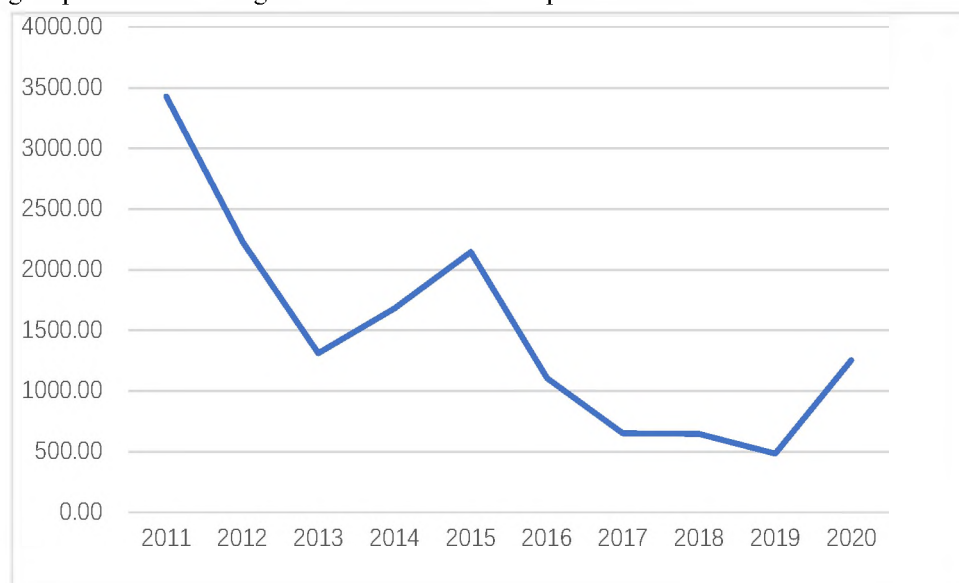
Figure 2. GHG Emissions
