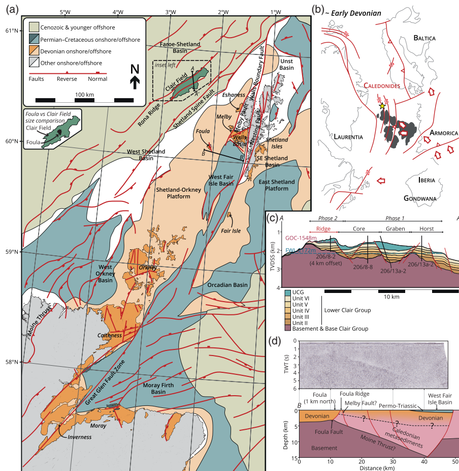
Fig. 1. (a) Regional map of the Orcadian Basin study area highlighting the Clair Field. Inset shows a simple map comparing the known extent of the Clair Field (green) in comparison with the size of the island of Foula (black). (b) Devonian palaeogeography and simplified reconstruction of the North Atlantic region; the approximate location of Shetland is shown by the yellow star. (c) North-south cross-section through the Clair Field; location of section shown in part (a). (d) WNW-ESE seismic reflection section (upper panel) and interpretation (lower panel) through the Foula Ridge and West Fair Isle Basin; location of section shown in part (a). Source: part (a) modified after Dichiarante et al. (2016) and Oil and Gas Authority (2019); part (b) modified after Dewey and Strachan (2003) ; part (c) modified after Barr et al. (2007) and Ogilvie et al. (2015) .
