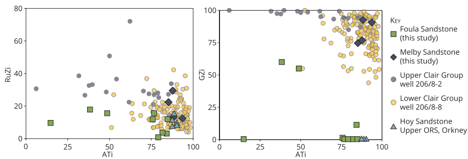
Fig. 12. Heavy mineral provenance relationships between the Foula Sandstone Group, the Melby Formation of Shetland, the Hoy Sandstone of Orkney, and the Lower and Upper Clair Groups of the Clair Field. ATI, apatite:tourmaline index; RuZi, rutile:zircon index; GZi, garnet:zircon index. Source: Morton and Hallsworth (1994); Clair Field data from Morton et al. (2010).
