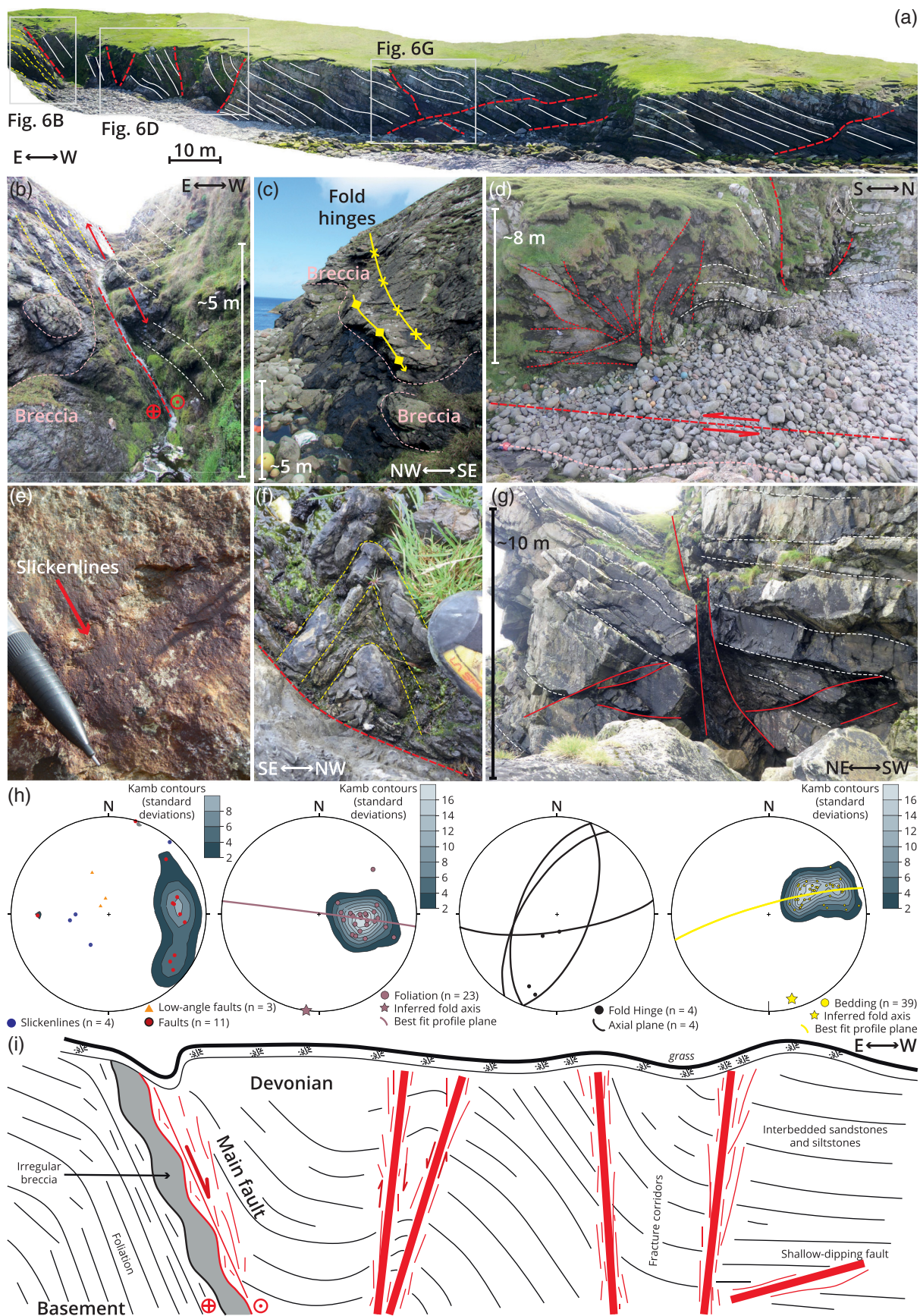
Fig. 6. Basement–cover relationships at Wurrwick [HT 396749 1140994]. (a) Annotated Virtual Outcrop Model of cliffs at Da Wast Banks o Wurrwick. (b) Principal slip surface of the Fould Fault with location of breccias. (c) SW-plunging folds in the footwall fault breccia. (d) SW-plunging folds and fractures in the hanging wall. (e) Close-up of fault plane showing sinistral oblique slickenlines. (f) Minor small-scale chevron folds within siltstones/mudstones in the hanging wall. (g) Fault zone in the hanging wall showing complex geometries and interaction of steeply dipping faults/fracture corridors and shallow bed-parallel faults. (h) Stereonets of major faults, foliation, fold axial planes and hinges, and bedding. Plotted as (Kamb) contoured poles to planes and mean planes shown as great circles. (i) Schematic summary diagram of the fault zone structure at Wurrwick covering the cliff section shown in part (a).
