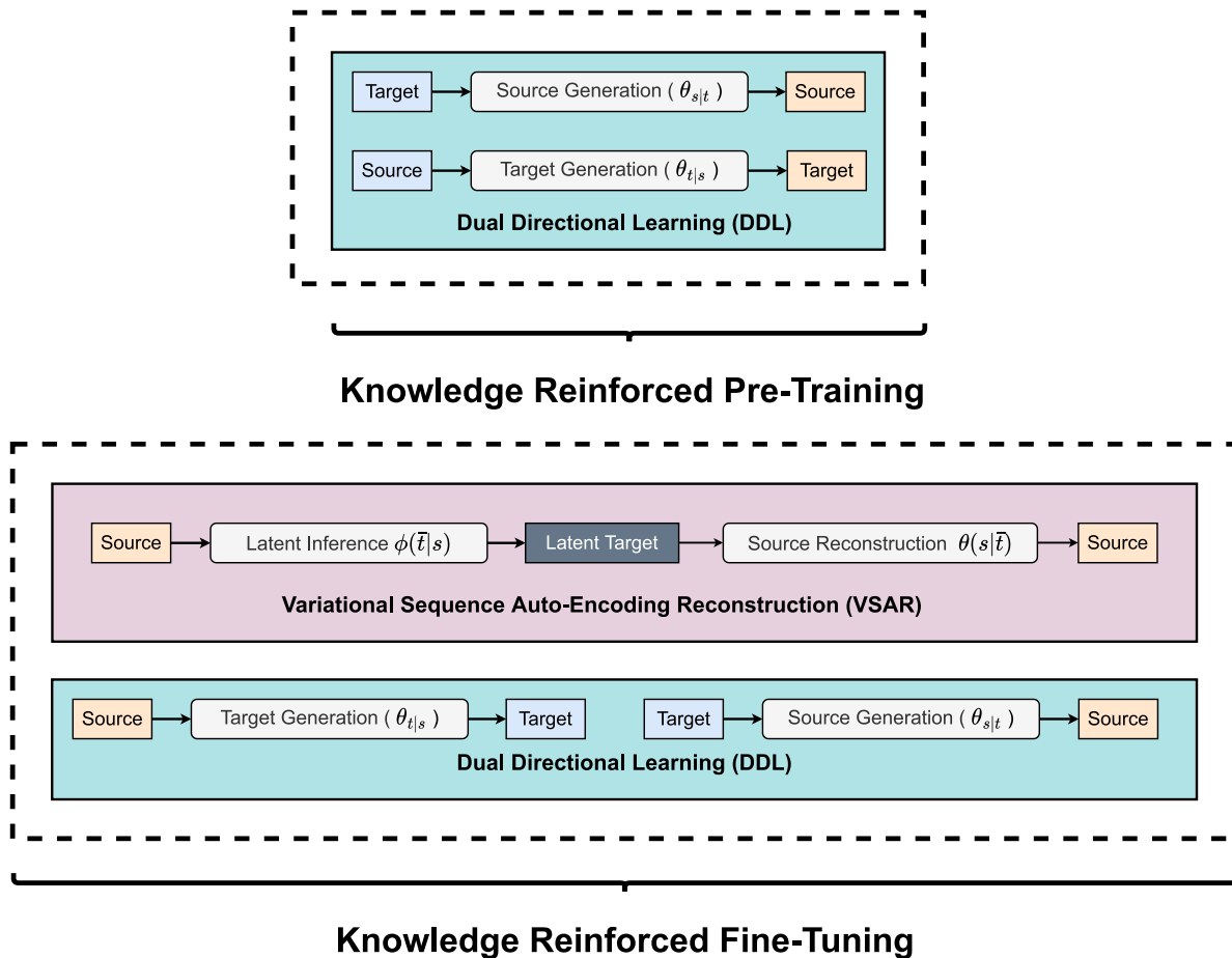
Fig. 2. Knowledge Reinforced Learning (KRL).
