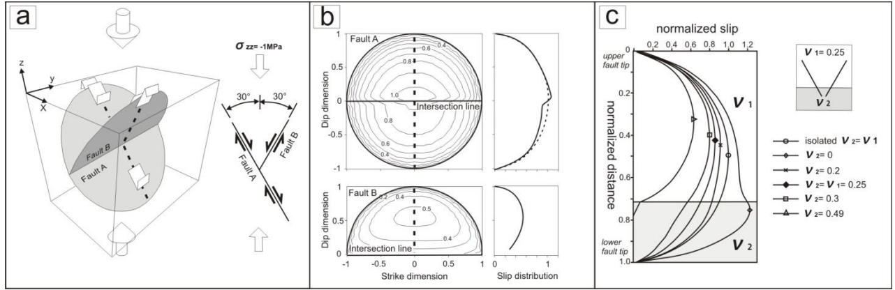
Figure 14. a. Configuration of the elastic boundary element model for conjugate normal faults with a “Y”-type geometry within a homogeneous whole elastic space, from Maerten (1999). b. Results of the modelled displacement distribution (Maerten, 1999). c. Calculated displacement distributions for conjugate normal faults with a “V”-type geometry located within a heterogeneous elastic material, derived from finite element method modelling (Young, 2001). Note the asymmetric slip distribution, skewed towards the upper fault tip, for models in which the fault intersection lies within a layer that has a higher Poisson’s ratio than the surrounding material (i.e. v_2 > v_1 ).
