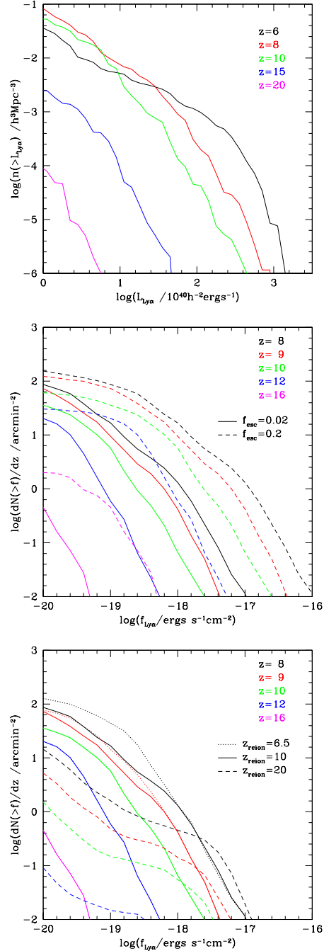
Figure 8. Predictions for the number of Ly \alpha emitters at very high redshifts. (a) The upper panel shows the evolution of the cumulative Ly \alpha luminosity function at 6 \leq z \leq 20 , for our standard model, with reionization redshift z_{\text{reion}} = 10 and Ly \alpha escape fraction f_{\text{esc}} = 0.02 . (b) The middle panel shows the predicted number counts per unit redshift interval per unit solid angle as a cumulative function of the Ly \alpha flux, for z_{\text{reion}} = 10 . Results are shown for two different escape fractions, our standard value f_{\text{esc}} = 0.02 (solid lines) and a larger value f_{\text{esc}} = 0.2 (dashed lines). We show number counts for selected redshifts falling within either the J,H or K atmospheric transmission windows, with different redshifts in different colours. (c) The lower panel shows the cumulative number counts as in (b), for our standard f_{\text{esc}} = 0.02 , and three different reionization redshifts, z_{\text{reion}} = 6.5 (dotted lines), 10 (solid lines) and 20 (dashed lines); where the dotted lines are not visible, they coincide with the solid lines. The number counts do not include attenuation by the IGM.
