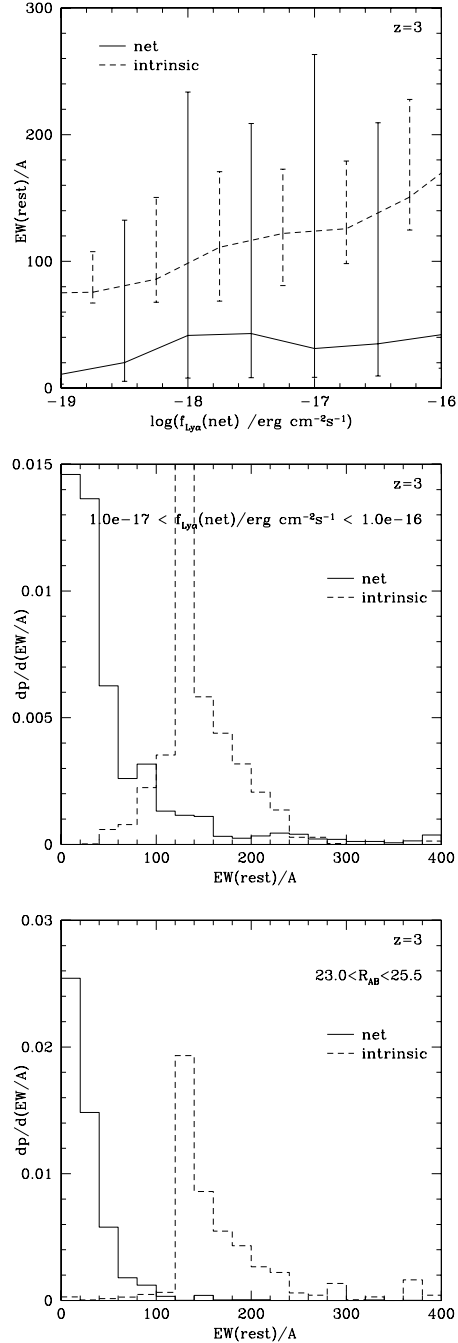
Figure 3. The predicted rest-frame equivalent width (EW) of the Ly \alpha emission line for galaxies at z = 3 . We show results both for the intrinsic EW, i.e. before including attenuation by neutral gas and dust in the galaxy, and for the net EW, i.e. after including the escape fraction for Ly \alpha photons and dust extinction of the stellar continuum - these are shown by dashed and solid lines respectively. In either case, the EW is considered as a function of the net Ly \alpha flux. (a) The upper panel shows the predicted median EW as a function of the net Ly \alpha flux. The error bars show the 10-90 percentile range at a given flux. (b) The middle panel shows the predicted distribution of EWs for galaxies with net Ly \alpha fluxes in the range 10^{-17} - 10^{-16} \text{ erg cm}^{-2} \text{ s}^{-1} . (c) The lower panel shows the predicted EW distribution for galaxies selected to have continuum magnitudes in the range 23 < R_{\text{AB}} < 25.5 .
