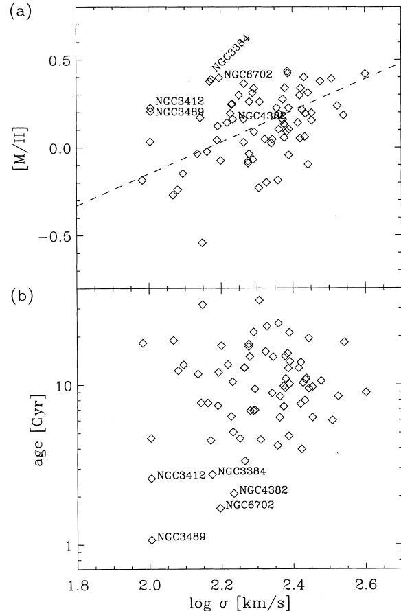
Figure 12. (a) The [\text{M}/\text{H}] - \sigma relation and (b) the \log \text{age} - \sigma relation for our sample of 72 galaxies. The ages and metallicities are derived from Fig. 8(a). The dashed line in panel (a) is not a fit to the data, but represents a slope of 0.9 dex in metallicity per dex in \log \sigma .
