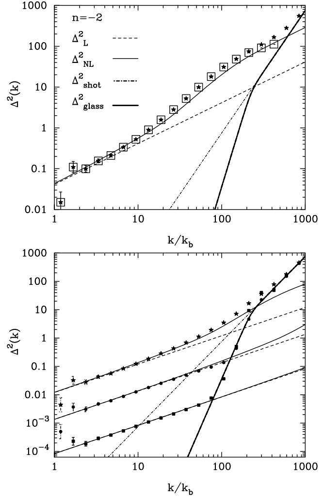
Figure 5. (Top) The glass-discreteness corrected (squares) and uncorrected power spectrum (stars) of the glass n = -2 simulation at an epoch a = 0.55 . We show the linear fluctuation spectrum (dashed line), which demonstrates that the box scale mode is still linear, the nonlinear spectrum according to the scaling formula of PD96 (thin solid line), a shot noise spectrum (dot-dashed line) and our two power-law discreteness model outlined in the text (thick solid line). (Bottom) Three epochs from the early stages of the same n = -2 simulation. From bottom to top epochs are a = 0.025 (squares), 0.1 (circles) and 0.3 (stars). This demonstrates that the discreteness spectrum does not evolve and also that the linear spectrum has been correctly established early on. Again, the lines are as in the top panel, with the thick solid line representing our fit to the discreteness spectrum.
