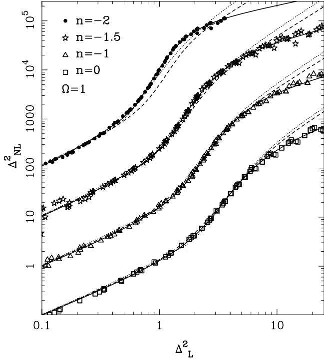
Figure 7. Nonlinear power plotted against linear power (points) for the four scale-free simulations. For clarity, the data have been separated from each other by one order of magnitude in the y -direction, with the n = 0 data untranslated. To determine the linear power given a nonlinear data point, the appropriate linear scale is required. In the HKLM method, this is found using the transformation k_L = [1 + \Delta_{NL}^2(k_{NL})]^{-1/3} k_{NL} . The solid line represents the fitting formula for the Einstein-de Sitter models presented in Appendix B; the dashed line represents the PD96 fitting formula; the dotted lines are the fits using the formula of JMW95.
