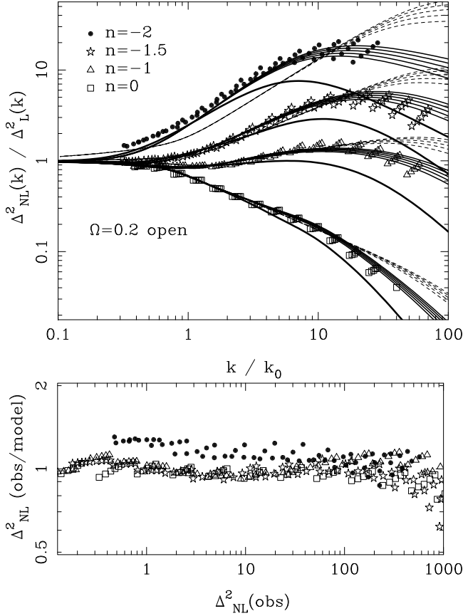
Figure 13. Top and bottom panels are similar to Fig. 12, but this time points represent open model data. Five epochs are shown; these are a = 0.6, 0.7, 0.8, 0.9, 1.0 . In terms of \Omega , these epochs correspond to: \Omega = 0.294, 0.263, 0.238, 0.217, 0.200 . The thick solid line represents the new halo-model based fitting to the scale-free data.
