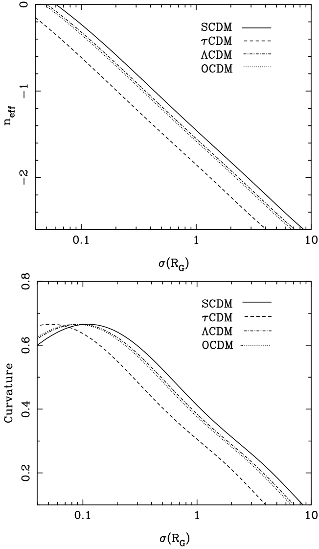
Figure 10. Variation of effective spectral index (top panel) and curvature (bottom panel) as a function of the rms fluctuation in Gaussian spheres of radius R_G , for the four cosmological models considered. Note the lower \sigma_8 values that corresponded to the big-box simulations has been assumed for the SCDM and \tau CDM models.
