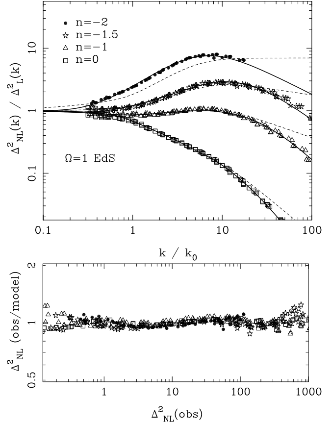
Figure 12. (Top) nonlinear power ratioed to the linear power as a function of wavenumber scaled in terms of the normalization wavenumber k_0 : where \Delta^2(k_0) = 1 . The data points are for the scale-free simulations; the solid lines represent the fits from the new halo based formula in Section 6.5; the dotted lines are PD96 fits. (Bottom) The goodness of the new fit. The y axis represents the ratio of observed nonlinear power to nonlinear power predicted by the halo based fitting function. The x axis is observed nonlinear power.
