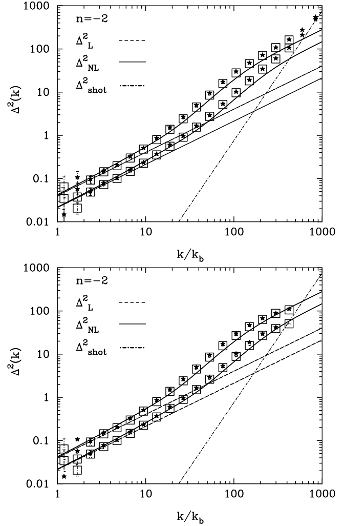
Figure 6. (Top) Comparison of discreteness uncorrected power spectra measured from the quiet start (squares) and glass start (stars) n = -2 simulations at epochs a = 0.4 and 0.55 . Line styles are as in Fig. 5. (Bottom) Comparison of discreteness corrected power spectra for the same outputs from the two simulations.
