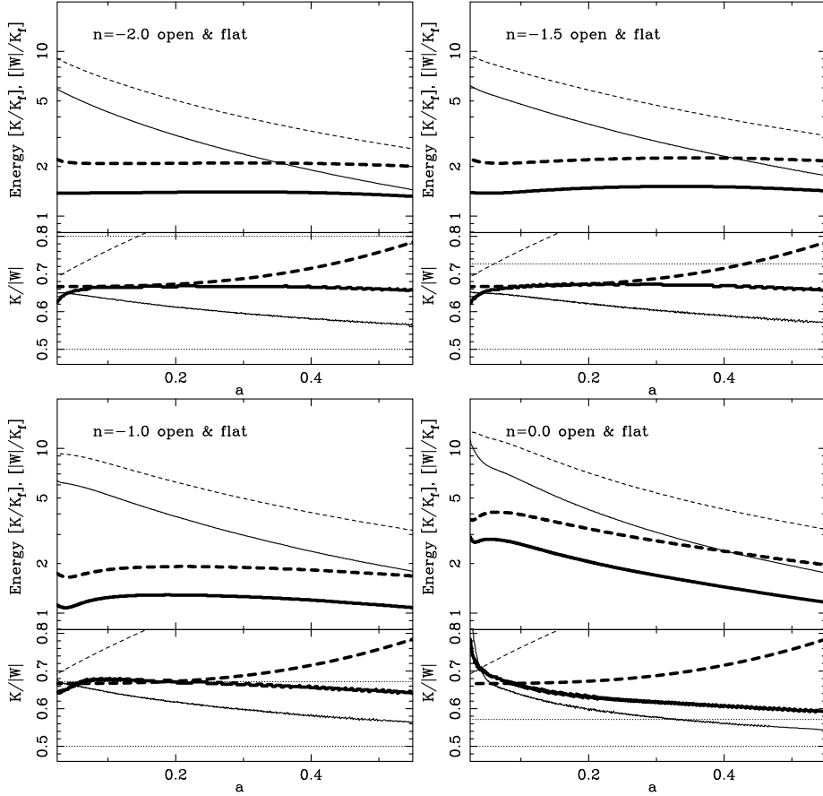
Figure 4. Similar to Fig. 3. However, this time for the \Omega < 1 power-law simulations. In the upper segment of each panel, thick lines represent flat models and thin lines represent open models. In the lower segment of each panel, solid lines represent the measured ratio, dashed lines denote the linear theory prediction according to equation (29) and dotted lines denote the \Omega = 1 ratio of 1 : 4/(n+7) (upper dotted), and the classical virial theorem ratio of 1/2 which becomes asymptotically valid (lower dotted). Again, thick lines represent flat and thin lines represent open universes.
