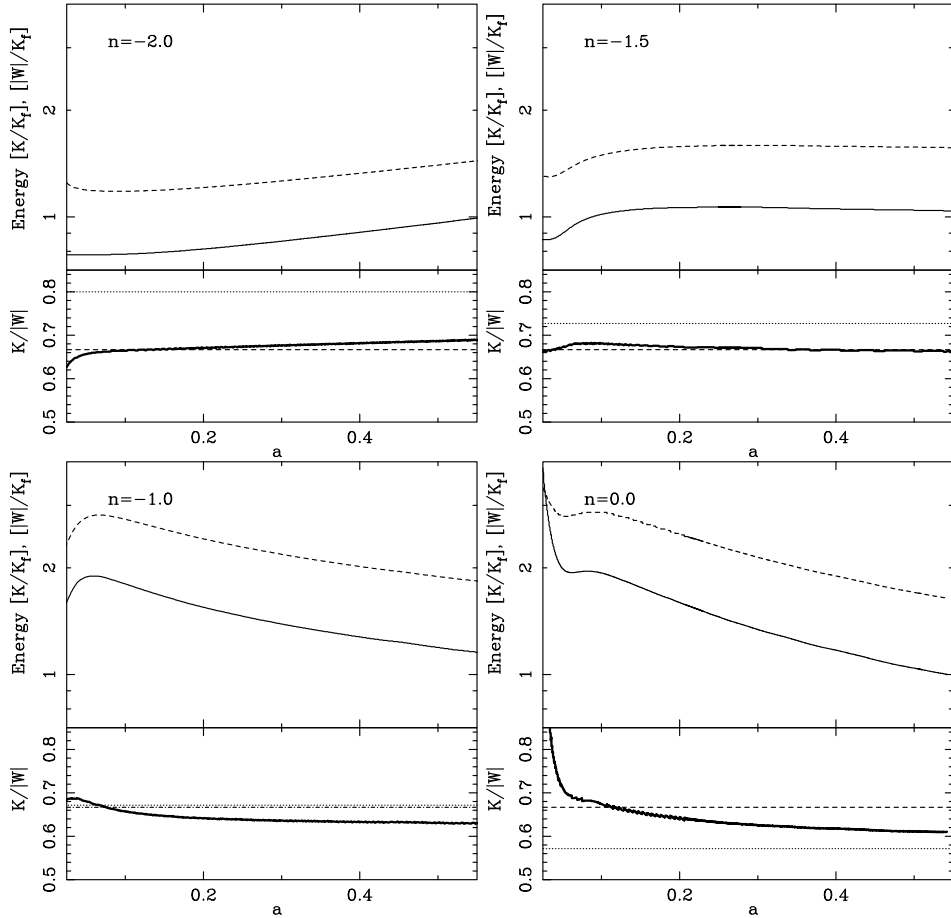
Figure 3. The upper segment of each panel shows the evolution of the total kinetic energy K (solid lines) and the total potential energy |W| (dashed lines) in the scale-free models, in units of the final kinetic energy K_f . The lower segment of each panel shows their ratio. During the linear phase of growth K and |W| should be in the ratio 2 : 3, as in equation (29); this is denoted by the dashed line. During self-similar growth K and W should be in the ratio 1 : 4/(n + 7) , as in equation (30); this is denoted by the dotted line.
