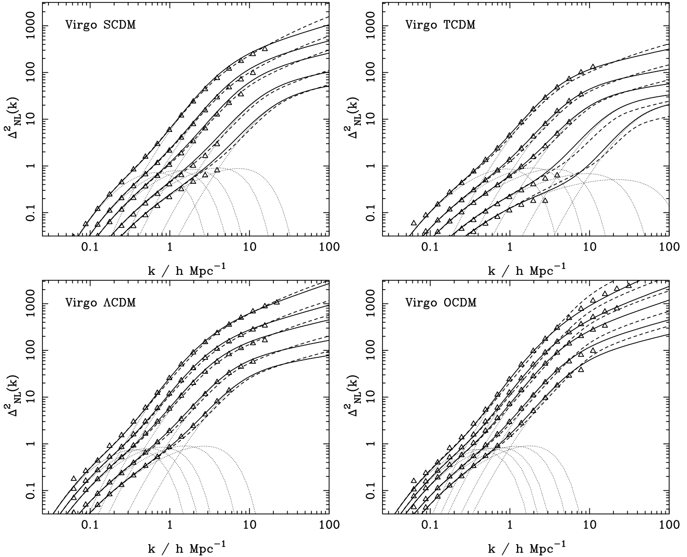
Figure 15. Power spectra for the four Virgo CDM simulations (J98) in large cosmological volumes, L = 239.5h^{-1}\text{Mpc} . Each panel shows the evolution of structure with redshift. The data points correspond, from low to high, to epochs z = 0, 0.5, 1.0, 2.0 and 3.0 . Note that only those points with a measured power above the discreteness spectrum are plotted. The solid line represents the new halo-model based fitting procedure, with dotted lines representing the decomposition into the self-halo and halo-halo terms; the dashed line is the PD96 fit.
