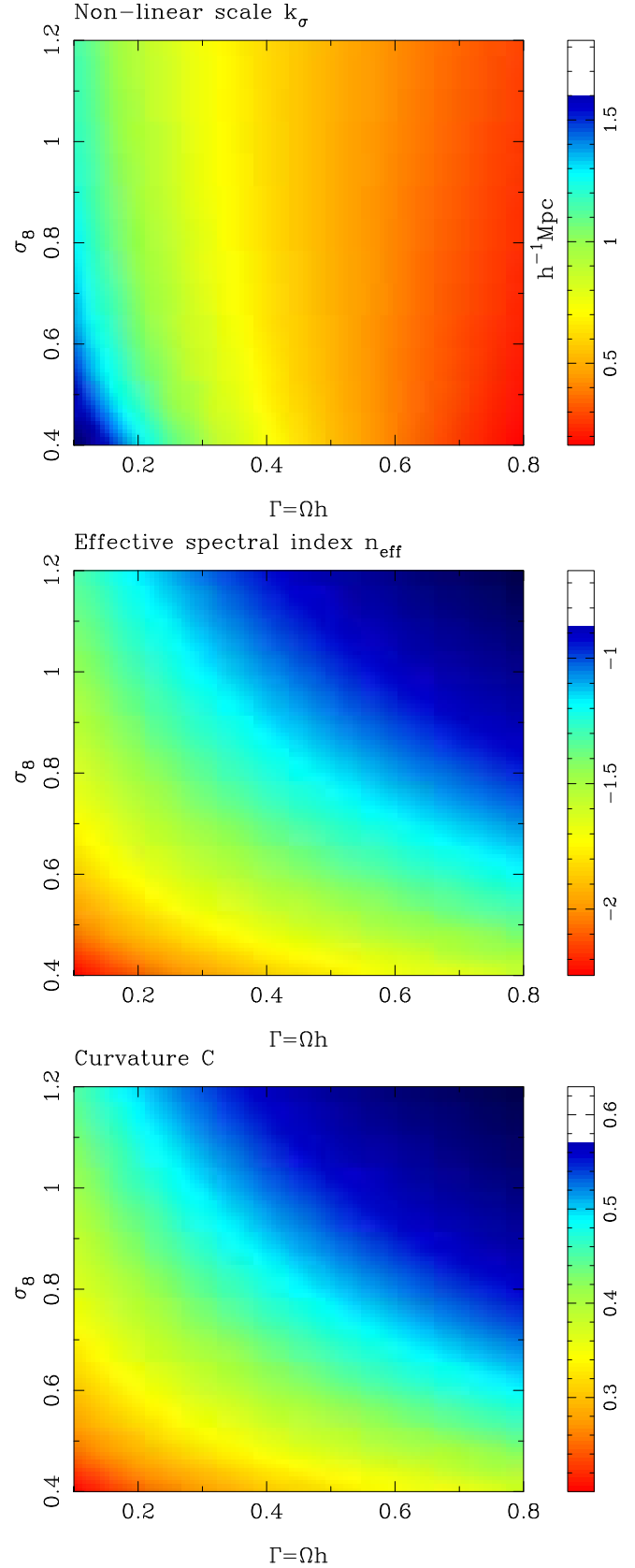
Figure 11. Dependence of the nonlinear wave-number k_\sigma (top panel), effective spectral index n_{\text{eff}} (middle panel) and curvature parameter C (bottom panel) on the shape parameter \Gamma and normalization \sigma_8 of the linear power spectrum. The parameters n_{\text{eff}} and C are degenerate under \Gamma and \sigma_8 . This degeneracy is, however, broken by the nonlinear wavenumber.
