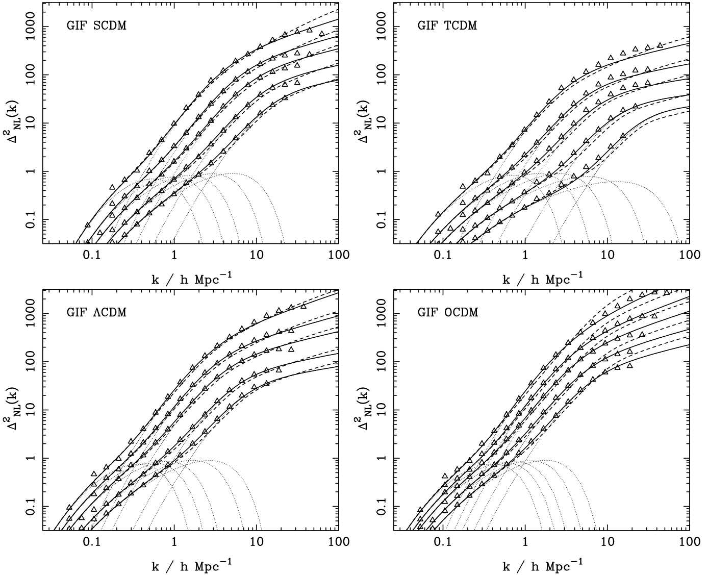
Figure 16. Same as for Fig. 15, but this time for the smaller box GIF simulations.
