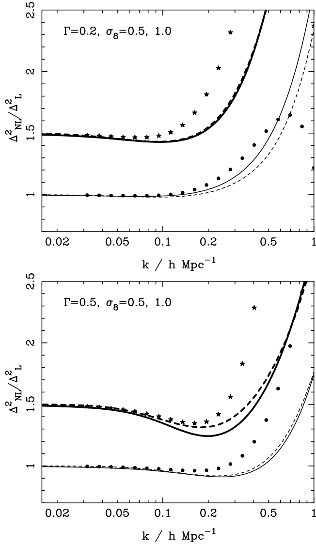
Figure 17. Comparison to perturbation theory. The top panel shows the ratio of the evolved power to the linear power for two CDM models with \Gamma = 0.2 , but with different normalizations. The model with \sigma_8 = 1 . has been translated by a factor of 0.5 in the y -direction. The points represent perturbation theory; the thick solid line is this work; the dashed line represents PD96. The bottom panel is the same as the top, but with \Gamma = 0.5 .
