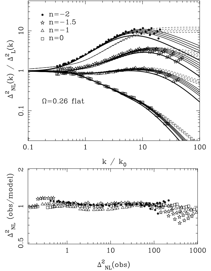
Figure 14. Top and bottom panels are similar to Fig. 12, but this time points represent \Lambda model data. Four epochs are shown; these are a = 0.7, 0.8, 0.9, 1.0 . In terms of \Omega , these epochs correspond to: \Omega = 0.505, 0.407, 0.325, 0.260 . Again, the thick solid line represents the fit to the scale-free data.
