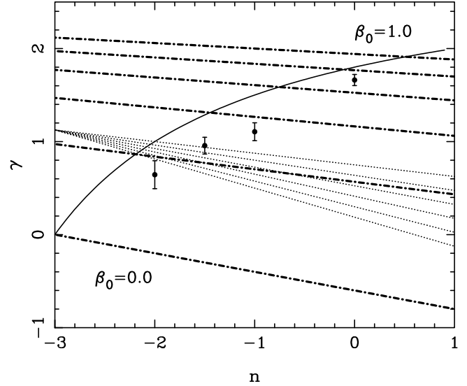
Figure 9. Nonlinear slope of the power-spectrum [\Delta^2(k) \propto k^\gamma] versus spectral index. Points are measured from the scale-free simulation power-spectra. The solid line represents the stable-clustering prediction. The dot-dash lines correspond to the predictions of the halo model (Ma & Fry 2000b), with an assumed \alpha = 0.4 and 0.0 \leq \beta_0 \leq 1.0 . The dotted lines correspond to the halo model prediction with \beta_0 = 0.25 and 0.4 \leq \alpha \leq 1.0 .
