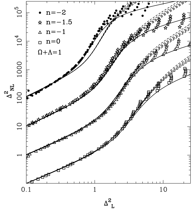
Figure 8. (Top) HKLM plot for the open models. (Bottom) HKLM plot for the flat low-density models with a cosmological constant. Again, for clarity, the data have been separated from each other by one order of magnitude in the y -direction, with the n = 0 data untranslated. For each model five epochs are shown, these are: a = 0.6, 0.7, 0.8, 0.9, 1.0 , with the lowest locus for each model corresponding to the a = 0.6 epoch. In terms of the mass density parameter of the universe, these epochs correspond to: \Omega = 0.294, 0.263, 0.238, 0.217, 0.200 for the open models and \Omega = 0.619, 0.505, 0.407, 0.325, 0.260 for the \Lambda models. As in Fig. 7 the solid lines represent the fitting formula for the Einstein-de Sitter models presented in Appendix B; the dashed lines represent fits from the PD96 function.
