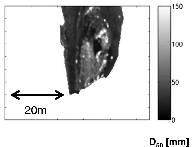
Figure 5. Example of a grain size map calculated with the optimal method, local semivariance, and 33 pixel \times 33 pixel (i.e., 99 cm \times 99 cm) sampling window, applied to the image in Figure 1a.
