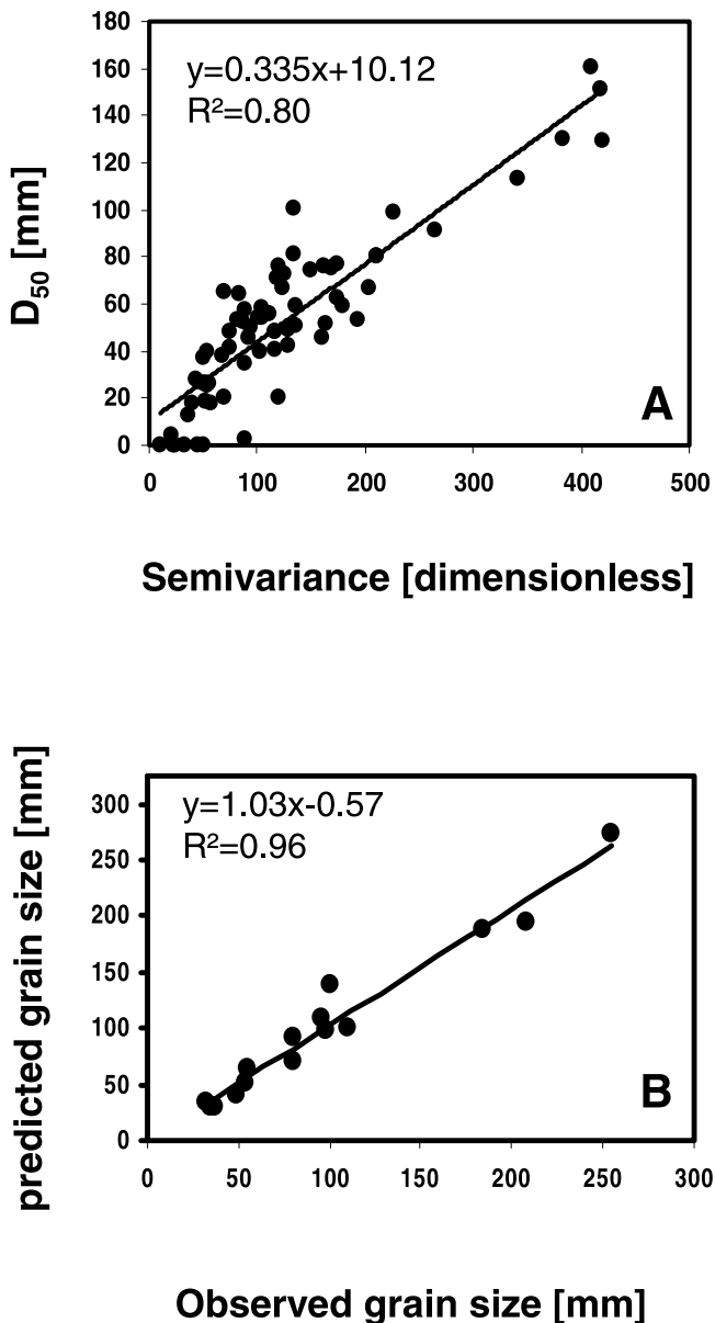
Figure 4. Regression plots showing the calibration and validation results of the semivariance method with a 33 pixel \times 33 pixel window applied to 3 cm resolution imagery. (a) Calibration relationship of median diameter ( D_{50} ) versus semivariance. (b) Validation relationship of predicted versus observed median grain sizes ( D_{50} ) obtained from an independent data set.
