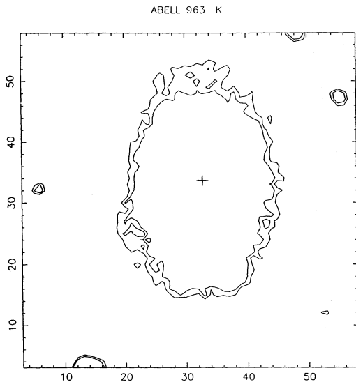
Figure 5. IR 2\text{-}\mu\text{m} image of the A963 cluster core displayed to reveal the detection of the N arc at a contour of \mu_K = 22.0 mag arcsec ^{-2} . The field is 36 \times 40 arcsec ^2 with the same orientation as in Fig. 1. The centre of the cD galaxy is marked with a cross.
