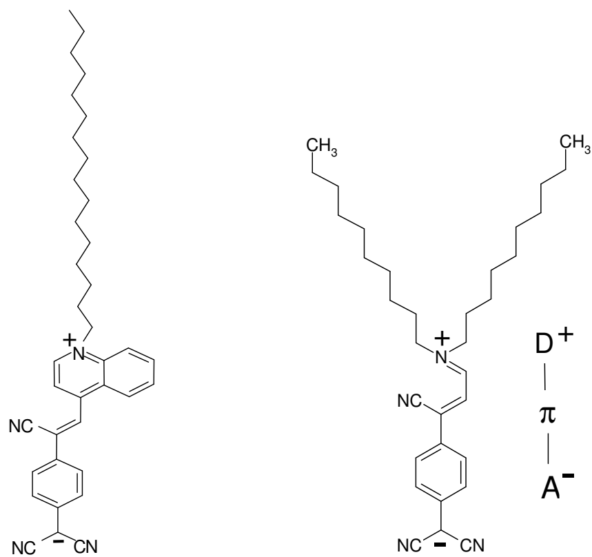
C_{16}H_{33}Q^+-3CNQ^- , molecule 1 [10, 11]
