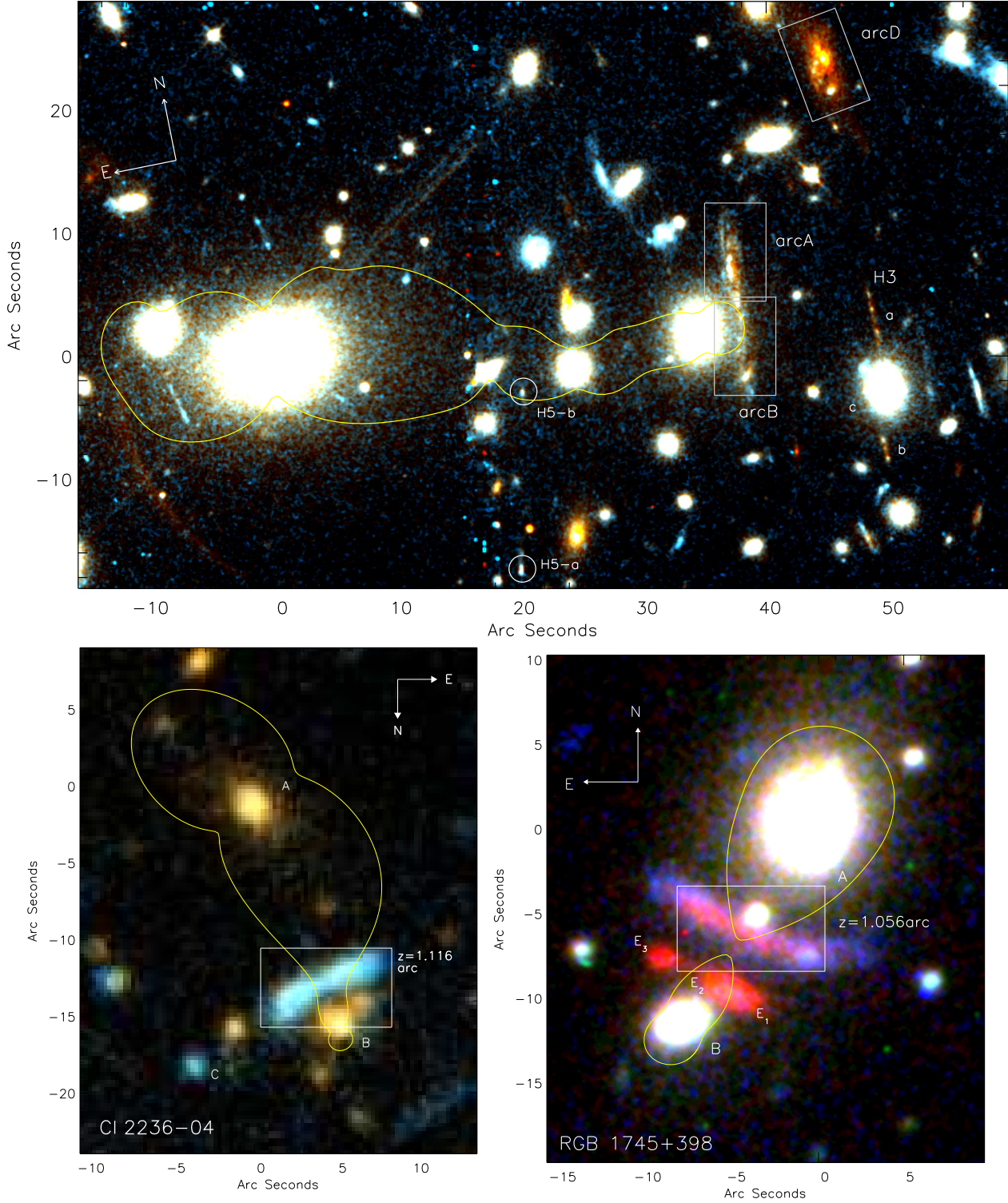
Figure 1. Finding charts for the IFU observations. Top: True colour HST VI image of the lensing cluster A2390 at z=0.228 with the GMOS IFU field of view overlaid on the three z \approx 1 arcs. The yellow curve is the z=0.912 critical curve calculated from the best-fit lens model of this cluster (§3.2.2; see also Fig. 3). We also label the z=4.04 and z=4.05 multiple-image systems that were used to constrain the lens model: H3-a/b/c and H5-a/b respectively. Lower left: True colour ground-based BVR image of the lensing cluster Cl 2236-04 with the GMOS IFU field of view overlaid on the z=1.116 arc. The brightest two cluster galaxies are labelled A and B, and the z=1.334 source discussed by Kneib et al. (1994) is labelled C. We also show the z=1.116 critical curve in yellow. Lower right: True colour ground-based BRK image of the lensing cluster RGB 1745+398 with the GMOS IFU field of view overlaid on the z=1.056 arc and the z=1.056 critical curve shown in yellow. The multiply-imaged ERO at (-5'', -9'') has a redshift of z=1.11 \pm 0.05 (§2.4) and is labelled E_1 , E_2 and E_3 .
