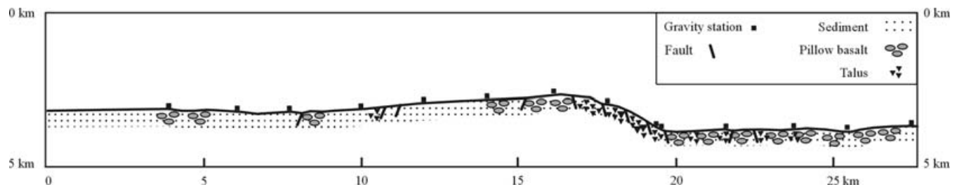
Figure 3. N–S profile produced from the three dives (12–14) across the E–W ridge, showing depth, seafloor lithology, and positions of gravity stations. North to the left. No vertical exaggeration.
