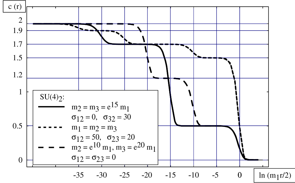
Figure 4: The TBA scaling functions for the SU(4)_2/U(1)^3 HSG model.
