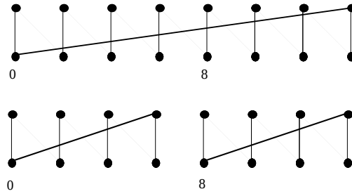
Figure 2: The posets \mathbf{C}_{16} and \mathbf{C}_8 \dot{\cup} \mathbf{C}_8 .
