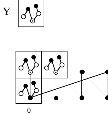
Figure 3: A coloured poset \mathbf{Y} , and a partial view of the poset \mathbf{S} . Darkened vertices in the copies of \mathbf{Y} are in the domain of \psi .
