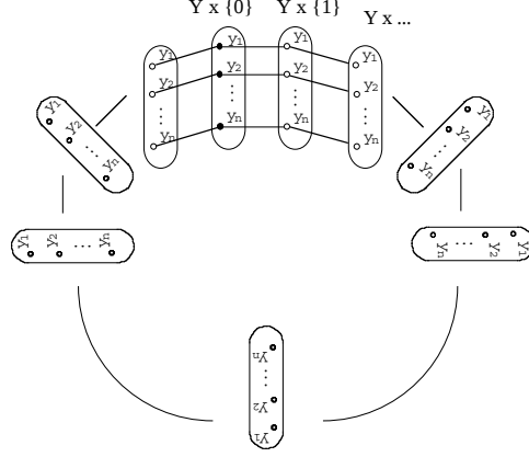
Figure 1: A partial view of the coloured graphs \mathbf{Y} glued to the n cycles \mathbf{C}_l .
