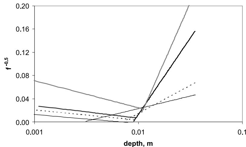
Figure 4. Summary of RMA regression lines for overland flow, similar to Figure 3, for the four surface covers: Eriophorum (thick black line), mixed Eriophorum/Sphagnum (dashed line), Sphagnum (thin black line), and bare (gray line).
