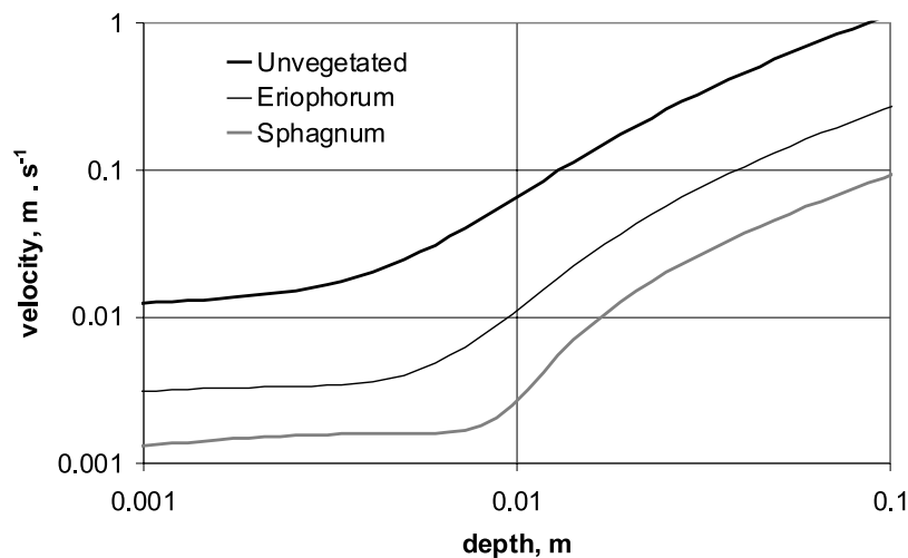
Figure 8. Modeled relationship between mean flow depth and velocity on a 10% gradient.
