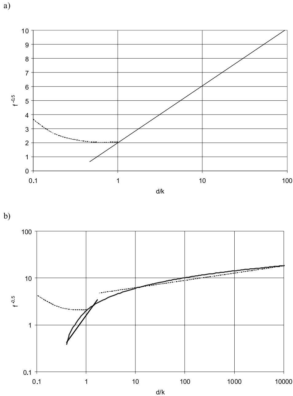
Figure 2. The relationship between Darcy-Weisbach roughness ( f^{-0.5} ) and the ratio of mean depth to effective roughness ( d/k ) from equation (4) (a) on a lognormal plot for comparison with later Figures 3–6 in this paper, with dotted curve sketching the relationship proposed by Lawrence [1997] for shallow depths ( f \sim d/k ), and (b) on a log-log plot. The dotted straight line indicates the fit over the range 10 < d/k < 10000 that is consistent with Manning's equation for which f^{-0.5} \sim (d/k)^{1/6} . The solid bold line indicates a fit in the region 0.5 < d/k < 2 that is more appropriate to overland flow, for which f^{-0.5} \sim (d/k)^{1.0} .
