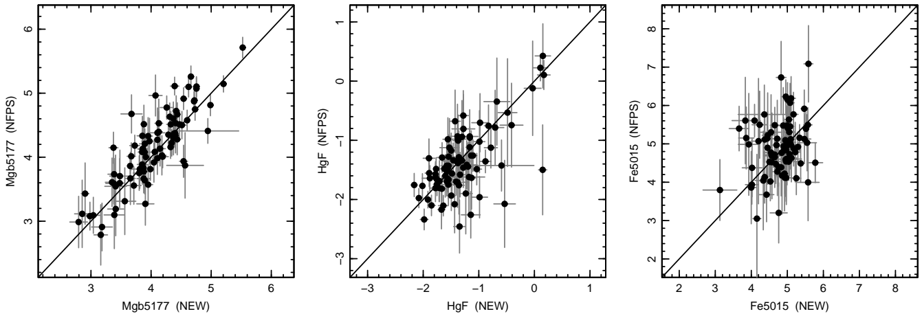
Figure 6. Comparison of the new index measurements with data from NFPS (Nelán et al. 2005), for three representative indices. There are 78 galaxies in common which meet our emission criterion ( \text{EW}(\text{H}\alpha) < 0.5 \text{ \AA} ). The line indicates equality.
