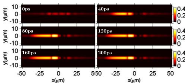
FIG. 3. (Color online) The same situation as in Fig. 2 but a potential is also applied to the third segment, such that the pump-polariton detuning there is \Delta_2=0.8 meV, and blocks the signal propagation along the polariton neuron.
