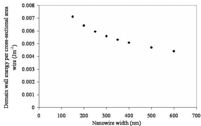
FIG. 3. Plot of domain wall energy per unit cross-sectional area as a function of nanowire width, deduced from OOMMF micromagnetic simulations. 8
