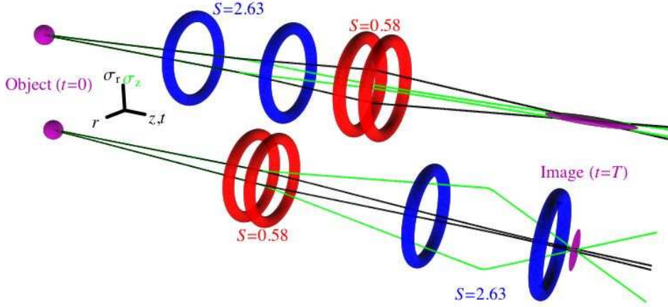
Figure 1. The principle of alternate gradient focusing. The upper image, Strategy AR, shows the evolution of the axial ( \sigma_z , green) and radial ( \sigma_r , black) cloud radii when an axially converging (radially diverging) lens precedes an axially diverging (radially converging) lens and leads to a sausage-shaped cloud ( \xi > 1 ). In the lower image, Strategy RA, the lens order is reversed, leading to a pancake-shaped cloud ( \xi < 1 ). The effects of gravity (in the -z direction along the coil axis) are not shown, but are included in simulations. Due to the time reversal symmetry of optics, the lens system also works backwards.
