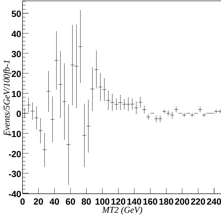
Figure 5.10: Subtracting opposite-flavour events passing the cuts from the passing same-flavour events. The scale is 100 \text{ fb}^{-1} .
