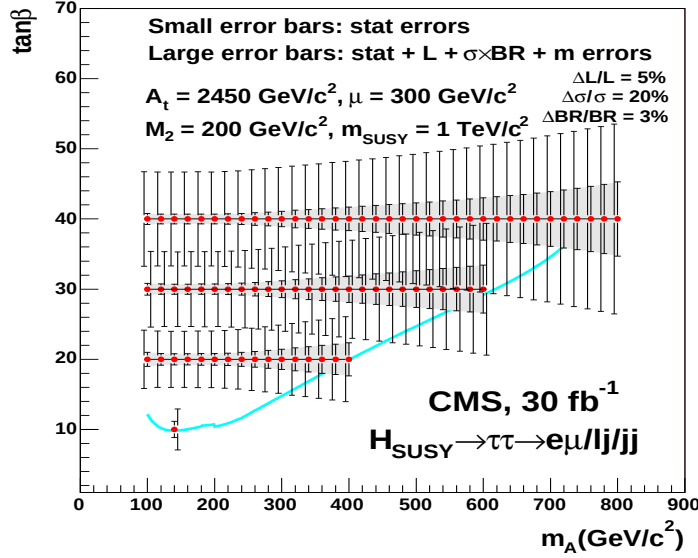
Figure 3.34: The uncertainty of the \tan \beta measurement shown as error bars. The small error bars and gray area show the statistical errors only. The large error bars exhibit the uncertainty if statistical errors, the mass measurement uncertainties, the luminosity uncertainty (5%) and the theoretical uncertainty of the production cross section (20%) and the branching ratio (3%) are taken into account. The solid curve corresponds to the 5\sigma -discovery contour.
