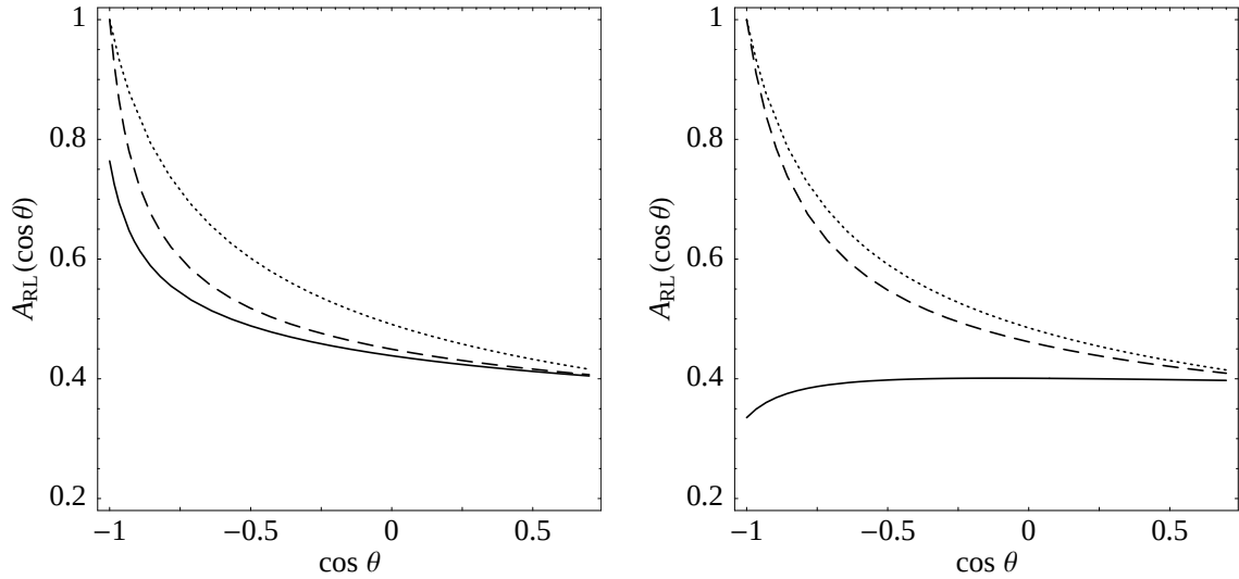
(c) m_X = 30 GeV.
