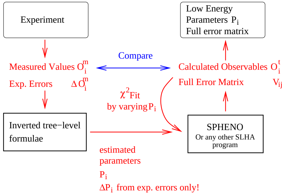
Figure 5.42: Iterative fit procedure
