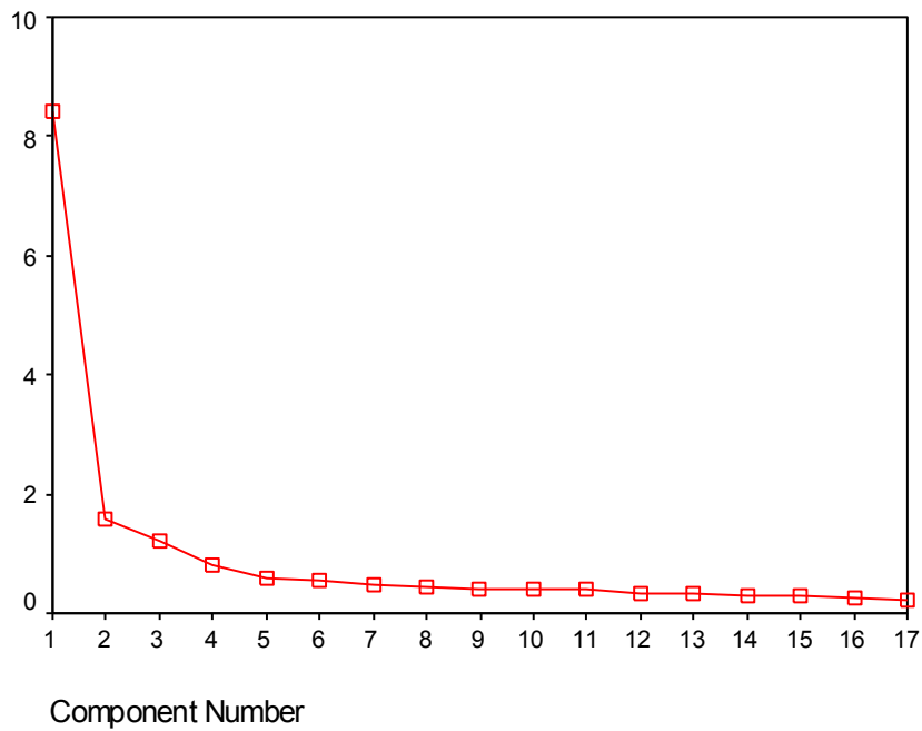
Scree Plot
