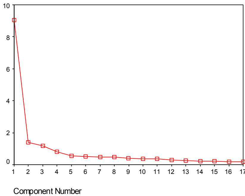
Scree Plot
