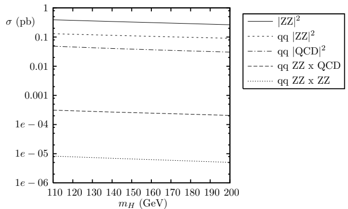
FIG. 3: The contribution to Hjj within the cuts of Eq. (4) from various tree level processes as a function of the mass of the Higgs boson. ZZ \times QCD and ZZ \times ZZ denote t \leftrightarrow u -channel interference terms.
