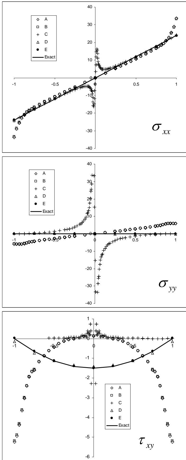
Figure 4: Plots of stresses across the section at x = 0 for the five analyses
