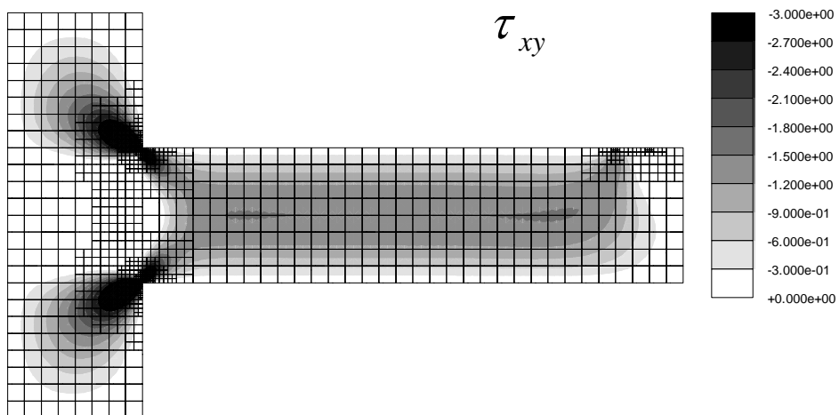
Figure 6: Stress contours and refined meshes for the realistic cantilever problem
