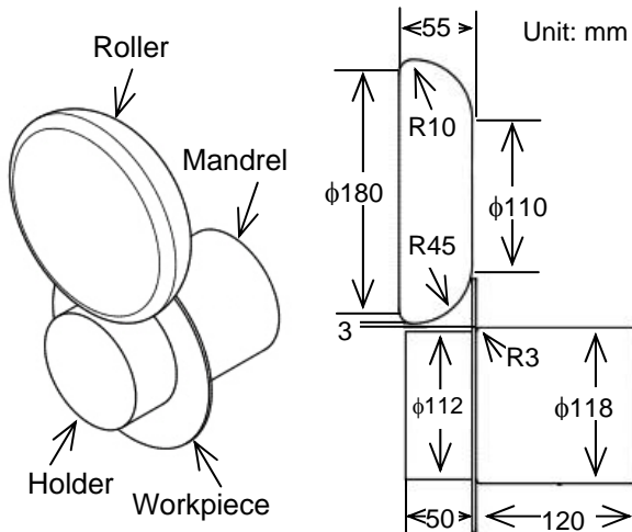
Figure 3. Geometry of FE analysis models.
