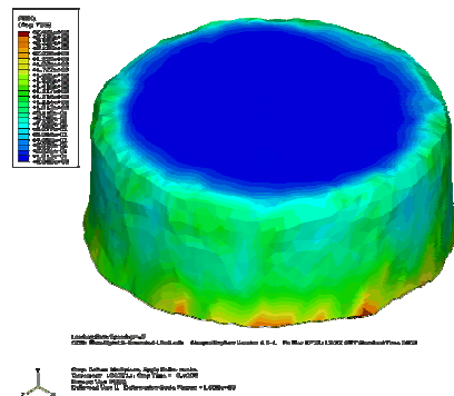
Figure 5. Equivalent plastic strain of Model 2 using load rate scaling.
