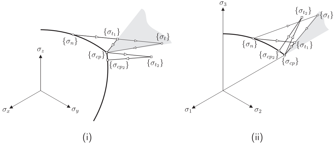
Figure 8: Modified reuleaux stress return crossing a corner. The figures illustrate a comparison between a single step and two specifically selected increments in (i) true stress space (ii) ordered principal stress space.
