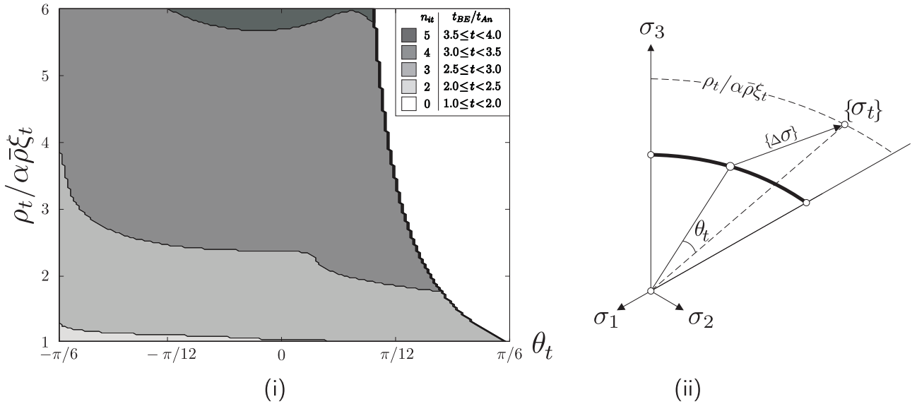
Figure 9: (i) Run time comparisons between conventional iterative backward Euler and the single-step analytical backward Euler stress returns (ii) geometric interpretation of a trial point in the run time analysis.
