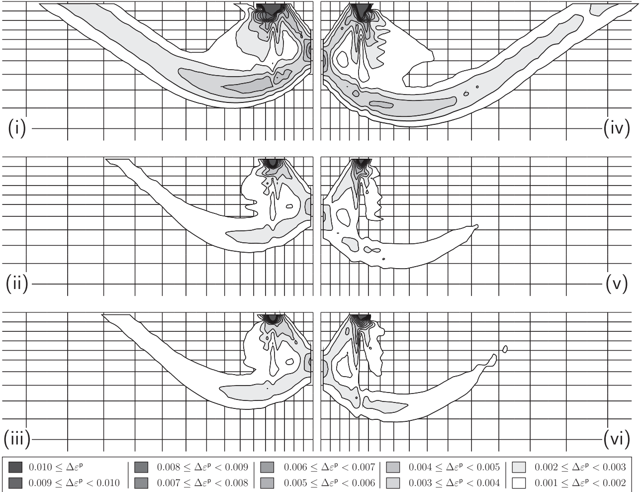
Figure 17: Rigid strip footing: contours of plastic strain increment, |\{\Delta \epsilon^P\}| , for the modified Reuleaux constitutive model during the final loadstep ( \Delta u = -1\text{mm} ). (i) small strain AF, (ii) small strain NAF, (iii) small strain NAF with cut-off, (iv) finite deformation AF, (v) finite deformation NAF, (vi) finite deformation NAF with cut-off.
