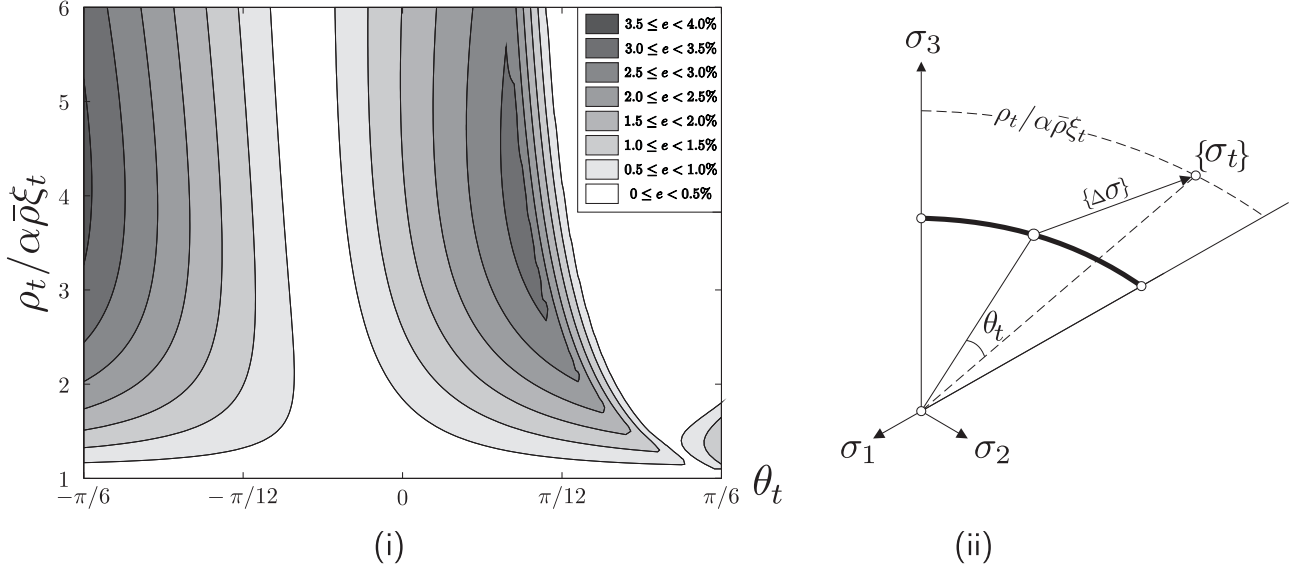
Figure 7: (i) Errors following from the single-step analytical backward Euler stress return (ii) geometric interpretation of a trial point in the error analysis.
