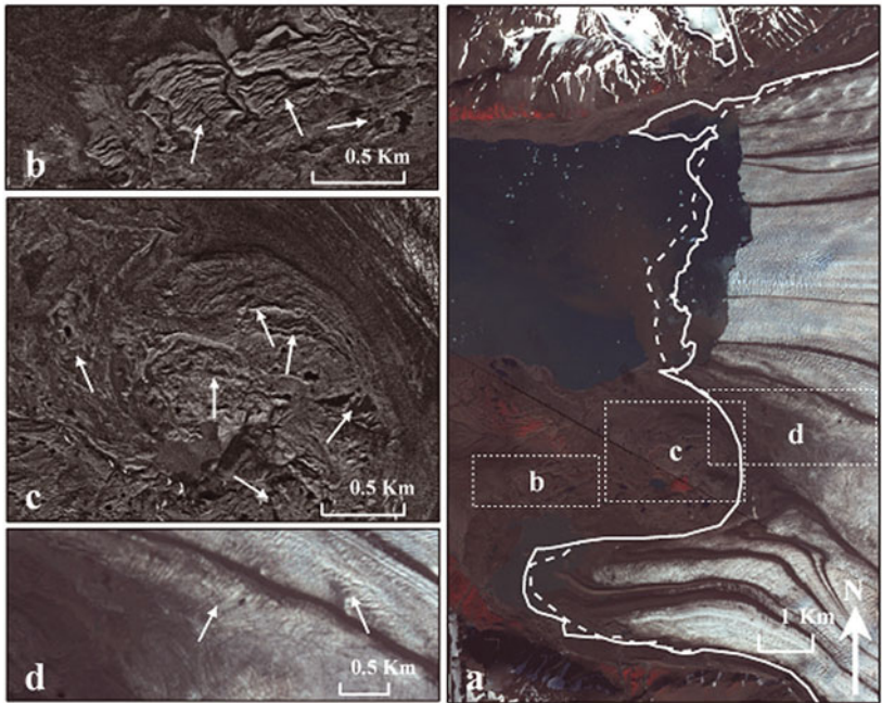
Fig. 2. Glaciological and geomorphological features identified on glacier No. 66, a type 1 surging glacier. (a) 2006 ASTER imagery. The solid white line represents the extent in 1976, and the dashed white line the extent in 1989, an advance of 600 m. Note the presence of looped moraines, extensive crevassing and the digitate nature of the terminus. The white arrows identify the following features: (b) thrust-block and hummocky moraines in 1976 ‘Hexagon’ imagery; (c) hummocky moraine, concertina eskers and crevasse-squeeze ridges in 1976 ‘Hexagon’ imagery; (d) deformed ice structures and shear margins in 2006 ASTER imagery.
