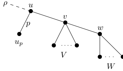
Figure 5: The vertices surrounding the edge (v, w) .
