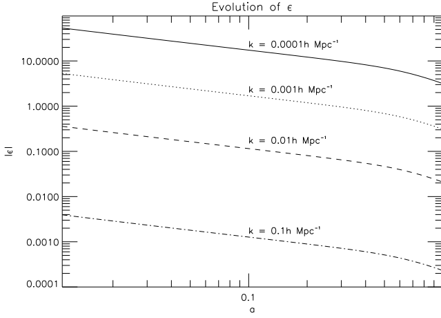
FIG. 2. The time-evolution of frame-independent quantity \epsilon \equiv \varepsilon + \sigma , for the model with f(T) = T - \mu^{2(1+n)}/(-T)^n and n = 0.1 , on different length scales, characterised respectively by k/(h \text{ Mpc}^{-1}) = 10^{-4} (solid curve), 10^{-3} (dotted curve), 10^{-2} (dashed curve) and 10^{-1} (dash-dotted curve).
