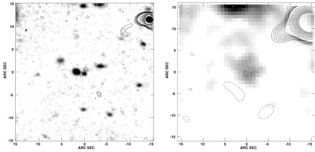
Figure 2. A multiwavelength view of LOCK350.1, a 3.9\sigma 350- \mu\text{m} blank-field source detected at RA = 10^{\text{h}}52^{\text{m}}43^{\text{s}}.2 , Dec. = 57^{\circ}23'9'' (J2000). The 30 \times 30 arcsec ^2 images are centred on the position of LOCK350.1. Left-hand panel: High-resolution (1.3 arcsec) 1.4-GHz contours ( -3, 3, 4, \dots, 10, 20, \dots, 100 \times \sigma ) from Biggs & Ivison (2006) overlaid on grey-scale archival R-band optical data. Right-hand panel: Low-resolution (4.2 arcsec) 1.4-GHz contours ( -3, 3, 4, \dots, 10, 20, \dots, 100 \times \sigma ) from Biggs & Ivison (2006) overlaid on grey-scale 24- \mu\text{m} data from Ivison et al. (2007).
