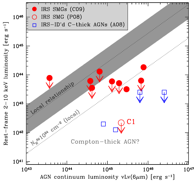
Figure 6. Rest-frame 2–10 keV luminosity derived from the X-ray vs. 6 \mu\text{m} luminosity derived from the mid-infrared power-law component fit (filled circles, where arrows indicate X-ray 3\sigma upper limits). For comparison, we overplot Spitzer -IRS z \sim 2 AGNs with optical spectroscopy from Alexander et al. (2008b; open squares) and the SMG C1 from P08 (open circle) which have properties suggesting they are Compton-thick. We have also overplotted the intrinsic (absorption corrected) X-ray-to-mid-infrared luminosity relationship for local AGNs (Lutz et al. 2004; the shaded region) and, assuming that it holds at high redshift, the combination of the observed (not corrected for absorption) X-ray luminosities and 6 \mu\text{m} luminosities of some of our objects suggests that they could be Compton-thick (see Figure 4 of Alexander et al. 2008b; the lower dotted line refers to the observed luminosity ratio expected for a typical AGN that is absorbed by N_{\text{H}} \simeq 10^{24} \text{ cm}^{-2} using the model presented in Alexander et al. 2005a). Note that C1 from P08 is also continuum-dominated in the mid-infrared, but it possesses a much lower L_{\text{X}} upper limit since it lies in a much deeper X-ray field.
