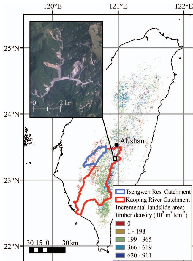
Fig. 2. Map of Taiwan, showing landslide areas identified as resulting from Typhoon Morakot, with color scale indicating the volume of timber accumulation based on the reported volumes for each forest type (Taiwan Forestry Bureau 1995). Inset shows FORMOSAT-2 imagery for identified region, illustrating the landsliding that stripped vegetation from hillslopes and supplied CWD directly to the river system. Black dot shows the location of Alishan, where the long-term precipitation record shown in Fig. 1 was collected.
