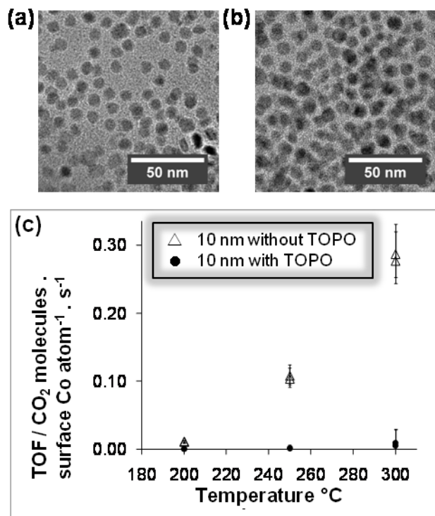
Figure 1. Showing TEM images of the 10 nm particles prepared using \text{Co}_2(\text{CO})_8 precursor and (a) without trioctylphosphine oxide (TOPO); or (b) using TOPO and (c) their corresponding activities for \text{CO}_2 hydrogenation reactions at various temperatures and 6 bar total pressure ( \text{CO}_2:\text{H}_2:\text{He} 1:3:0.5). Errors are estimates based on uncertainty in Co surface area for each sample from the ICP-AES and TEM measurements, duplicate catalytic runs are shown on the graph for each condition.
