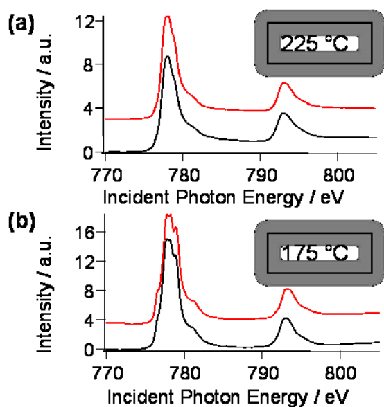
Figure 7. NEXAFS Spectra of the Co L-edge acquired in-situ during reduction of 2-D films of 10 nm Co nanoparticles deposited on silicon wafers (~50% coverage) in 1 bar H 2 using total electron yield detection and showing that both samples prepared with (red) and without (black) TOPO become reduced at very similar temperatures, being partially oxidized at 175 °C and almost fully reduced at 225 °C.
