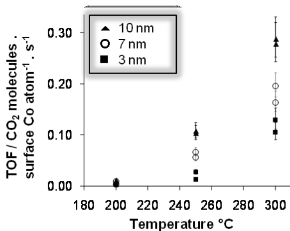
Figure 4. Showing activities for CO 2 hydrogenation reactions at various temperatures and 6 bar total pressure (CO 2 :H 2 :He 1:3:0.5) for 10, 7 and 3 nm Co nanoparticles prepared using TOPO free synthesis method to yield different particle sizes. Errors are estimates based on uncertainty in Co surface area for each sample from the ICP-AES and TEM measurements, duplicate catalytic runs are shown on the graph for each condition.
