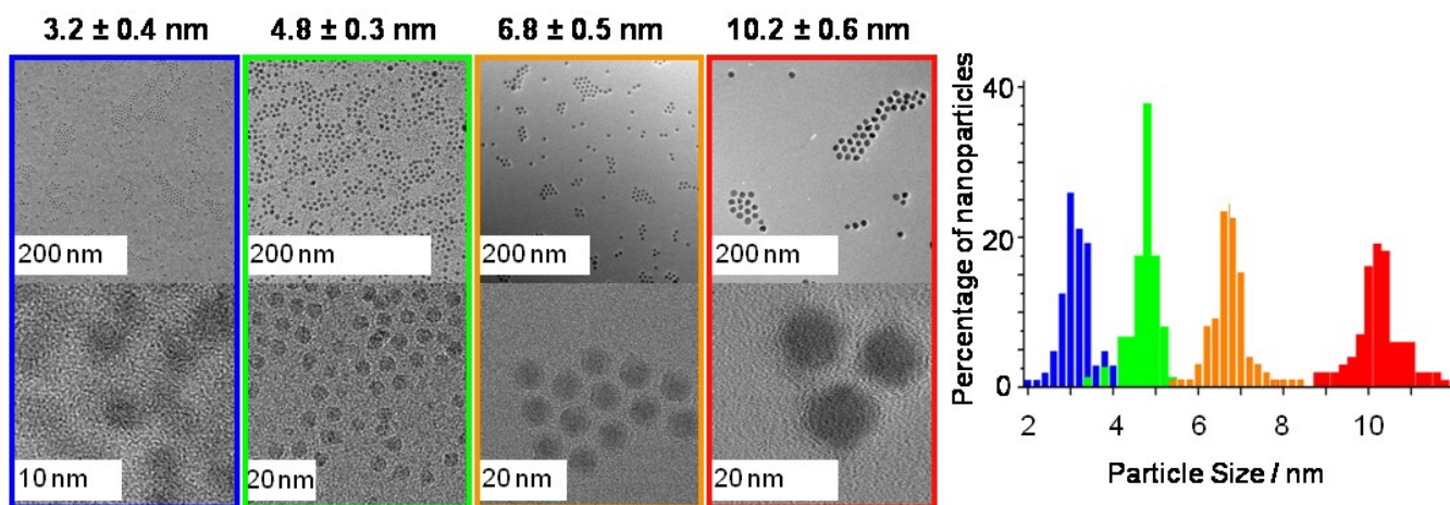
Figure 2. Typical TEM and HRTEM images of particles of four different sizes (3.2 nm; 4.8 nm; 6.8 nm and 10.2 nm) prepared without using TOPO and controlling particle size using variation in the temperature of the solution into which the \text{Co}_2(\text{CO})_8 is injected and the corresponding particle size distributions obtained from counting 200-300 particles.
