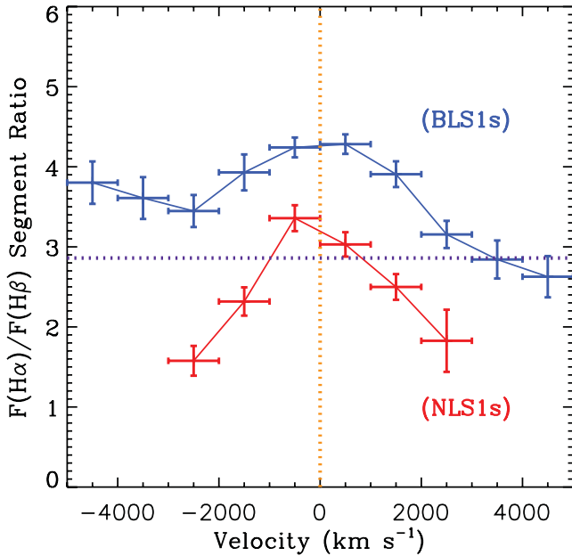
Figure 9. Balmer decrement changing across the Balmer line profile from +5000 to -5000 \text{ km s}^{-1} . Each data point represents the average decrement value in that segment with the vertical bar showing the \pm 1 standard error. Blue points show the results for the BLS1s, and red points show the results for NLS1s. However, due to the small line width of NLS1, the flux outside \pm 3000 \text{ km s}^{-1} for NLS1s is of low S/N; thus only the mean decrement values in the central \pm 3000 \text{ km s}^{-1} region were calculated and shown. The horizontal purple dotted line is a reference line at F(\alpha)/F(\beta) = 3 .
