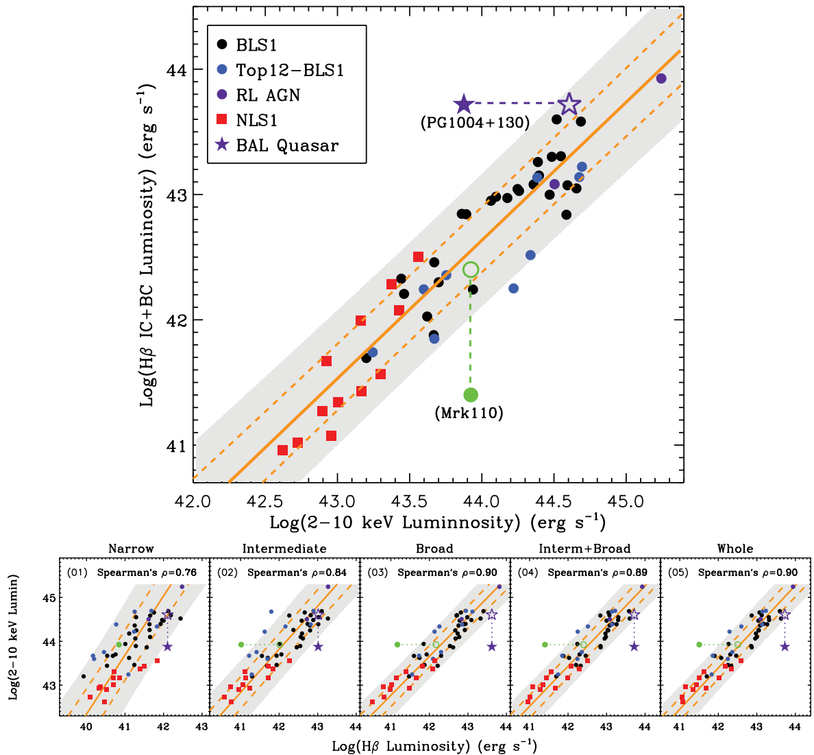
Figure 3. The luminosity correlation between Balmer line components and 2–10 keV. The upper figure shows the H\beta luminosity (NC-subtracted) versus L_{2-10\text{keV}} . The connected filled and empty purple stars indicate the position of PG 1004+130 before and after being corrected for 0.73 dex (Miller et al. 2006). The connected filled and empty green circles indicate different optical positions of Mrk 110 as calculated from the SDSS spectrum and the FAST spectrum (Landt et al. 2011). The solid orange line shows the linear regression line treating L_{2-10\text{keV}} as the independent variable, with the two dashed orange lines indicating the \pm 1\sigma region for new observations, and the shaded region showing the \pm 2\sigma region. The lower panels present the same type of correlations for different H\beta components, i.e. H\beta NC, IC, BC, IC+BC (or NC-subtracted) and the whole line. In each plot, Spearman's rank coefficients were calculated after excluding PG 1004+130 and Mrk 110. The regression coefficients are listed in Table B1 (see Supporting Information).
