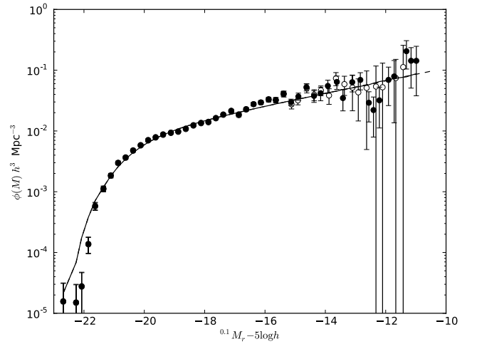
Figure 12. LF estimates in the r band for low-redshift galaxies ( z < 0.1 ) using the CMB reference frame (open circles) and the Tonry et al. (2000) multiattractor flow model (filled circles) using the SWML estimator. The solid and dashed lines show the best-fitting Schechter functions which are indistinguishable.
