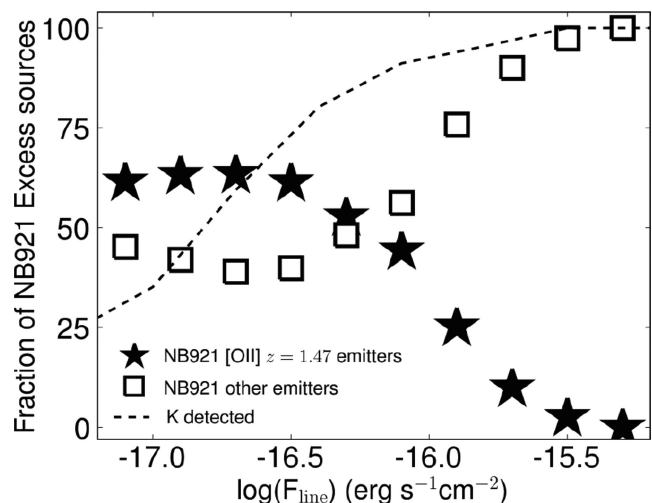
Figure 11. Fraction of [O II] and non-[O II] NB921 emitters (amongst those with K detections, allowing for a colour–colour separation) as a function of emission-line flux. A significant number of potential line emitters are not in the final [O II] colour-selected sample as they are not detected in the K -band imaging; the fraction of all emitters with a K detection is also shown.
