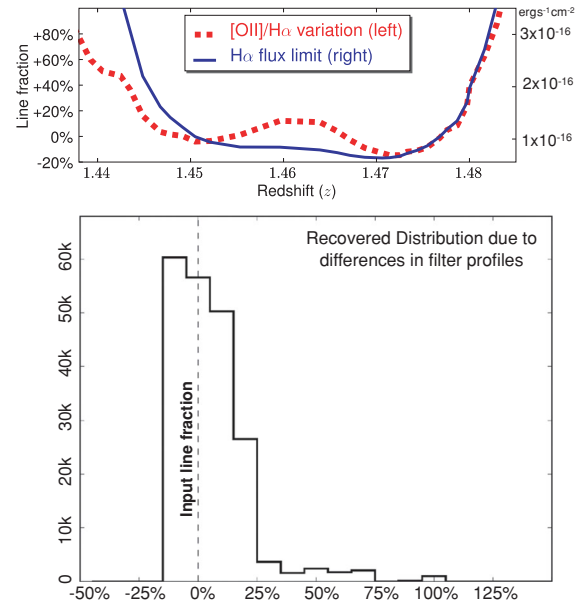
Figure 12. Top: the variation of the measured [\text{O II}]/\text{H}\alpha line ratio as a function of galaxy redshift due to the small differences in the transmission function of both filter profiles. Note that the flux limit (in units of \text{erg s}^{-1} \text{ cm}^{-2} ) also varies very significantly as a function of redshift, and thus line ratios are likely to be correct to within less than 20 per cent for the large bulk of the sample. Bottom: by using the \text{H}\alpha luminosity function to produce a population of galaxies distributed over a wider redshift range than the filter profile, it is possible to use both \text{NB}_H and NB921 filter profiles to study in a simple way the distribution of the ratio between the recovered and input line fractions. The results recover the input line fraction with 17 per cent standard deviation and with less than 1 per cent recovered with a line fraction increased by more than +50 per cent.
