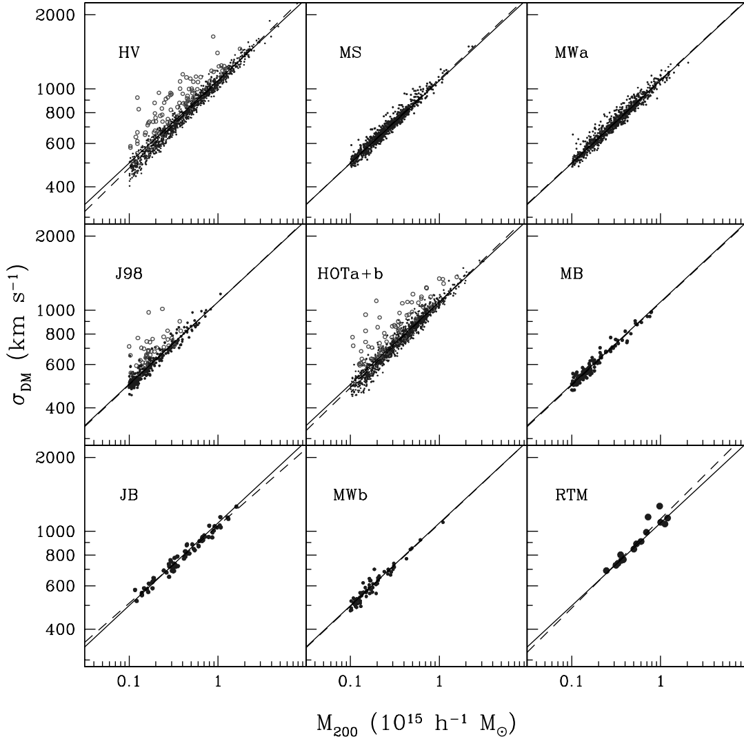
FIG. 2.—Dark matter halo virial relation for \Lambda CDM models, defined in Table 1, at z = 0 . Point styles are primary halos ( dots ) and satellites ( open circles ). One thousand randomly chosen halos are shown for samples larger than this size. The top two rows are N -body simulations of dark matter; the bottom row includes gas as a second, collisional fluid. The dashed line in each panel is the least-squares fit for that model (Table 4). The solid line in all panels is the global best-fit with parameters listed in Table 3. [See the electronic edition of the Journal for a color version of this figure.]
