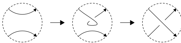
Fig. 5. A cobordism of Euler characteristic -1 inserting a positive crossing. The cobordism consists of a Reidemeister I move and a saddle move.
