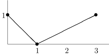
FIGURE 2. The Newton polygon of f \in \mathbb{F}_p[u_2^{\pm 1}][u_1^{\pm 1}] with respect to |\cdot|
