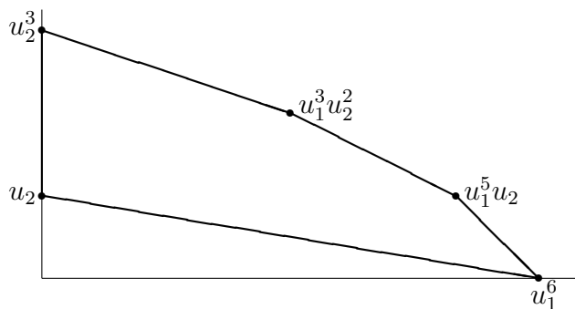
FIGURE 5. The support of a polynomial giving 4-fold mixing
