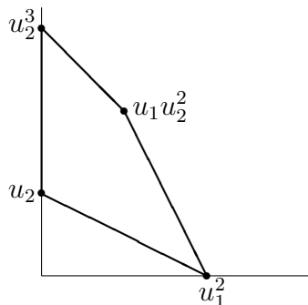
FIGURE 4. The support of a polynomial giving 3-fold mixing
